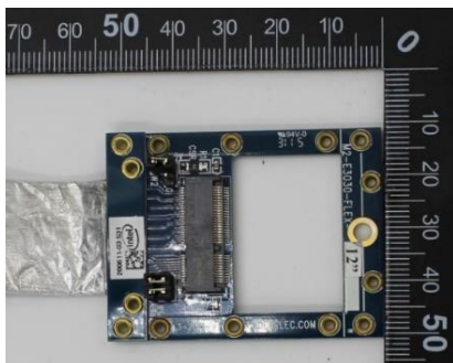
Extender board
