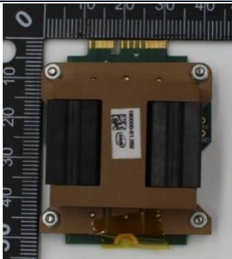
Extender board
