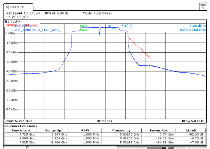
BE-NR-HIGH, SISO-B, 802.11ac80-VHT0, Ch171
