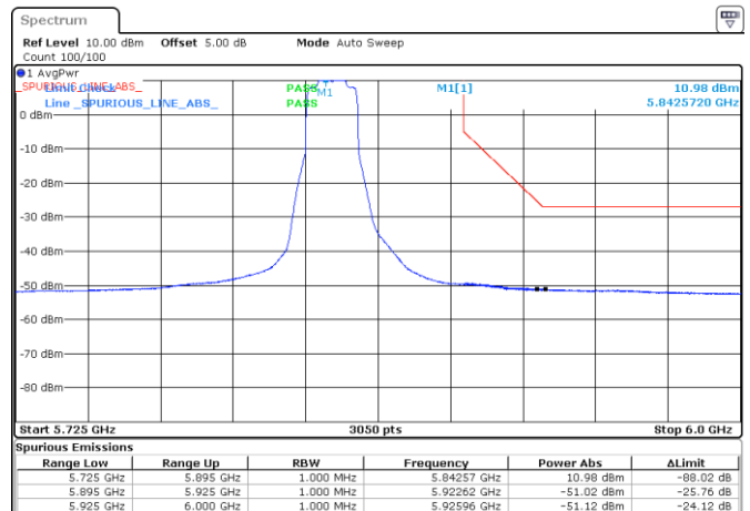
BE-NR-HIGH, SISO-B, 802.11ax20-HE0, Ch169
