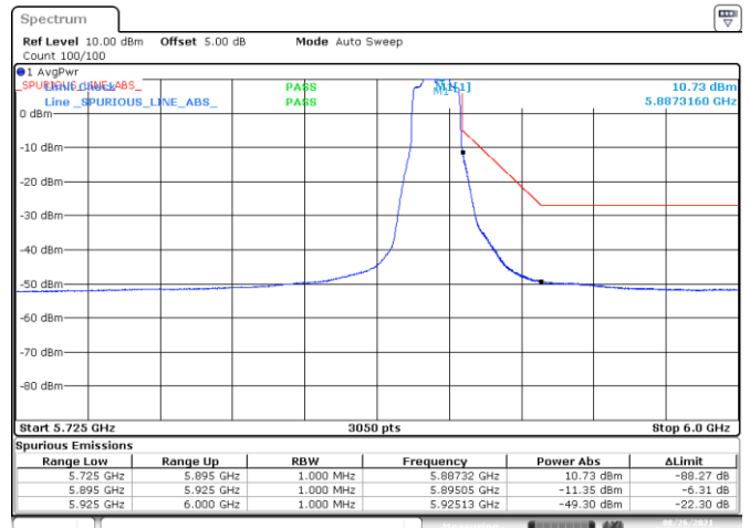
-BE-NR-HIGH, SISO-A, 802.11n20-HT0, Ch177
