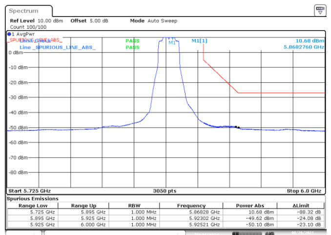
-BE-NR-HIGH SISO-A, 802.11n20-HT0, Ch173
