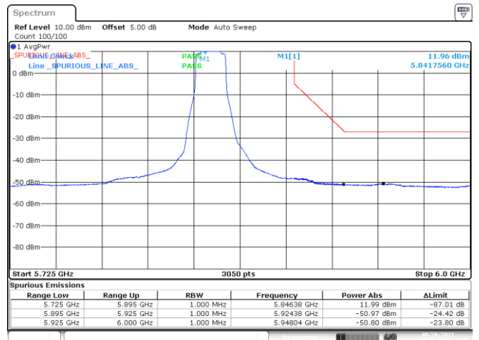
-BE-NR-HIGH, SISO-A, 802.11n20-HT0, Ch169
