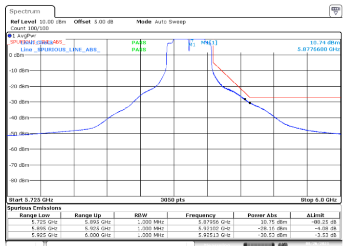
-BE-NR-HIGH, SISO-A, 802.11n40-HT0, Ch175
