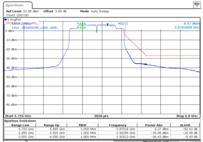
-BE-NR-HIGH, SISO-A, 802.11ac80-VHT0, Ch171
