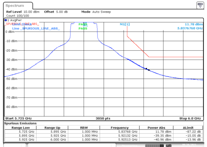
-BE-NR-HIGH, SISO-A, 802.11n40-HT0, Ch167
