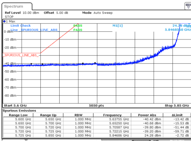
-BE-NR-LOW, SISO-A, 802.11ax20-HE0, Ch169
