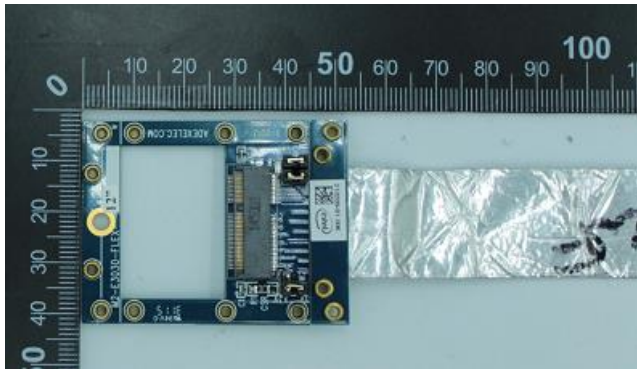
Antenna 1
