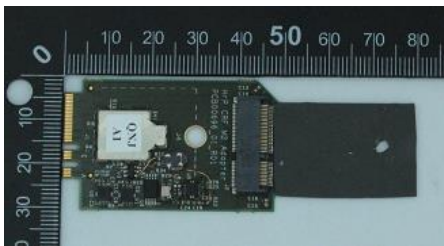
Extender board
