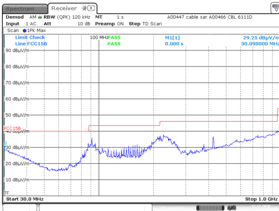
Plot 2 Pre-scan plot with peak detector. Radiated emissions from 30 MHz to 1000 MHz 2.4GHz mode
