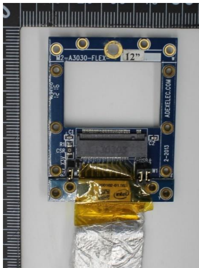
Socket front
