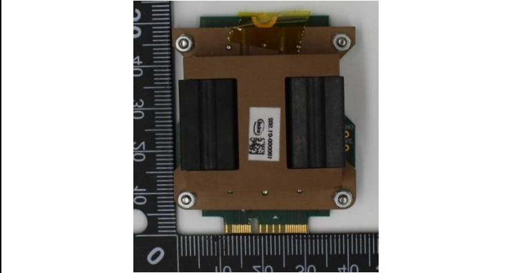
Main Antenna
