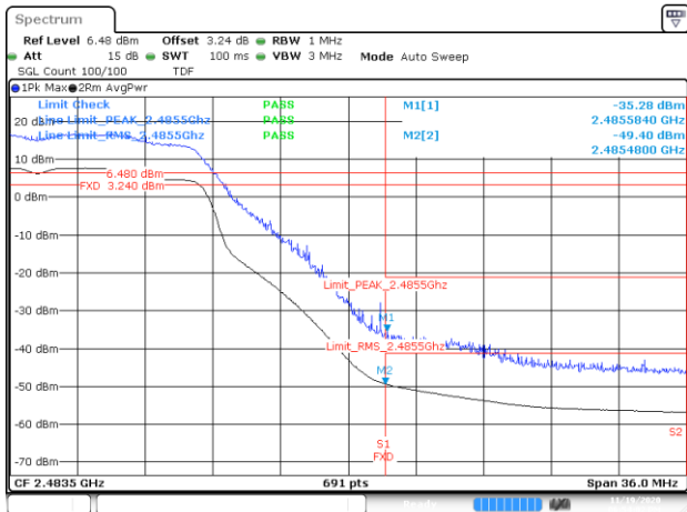
BE-R-HIGH, DIV-2, 802.11n20-HT0, Ch12
