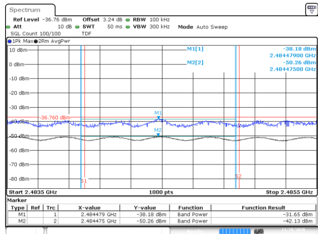
BE-R-HIGH-2MHz, DIV-2, 802.11n40-HT0, Ch9
