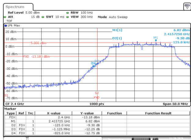
BE-NR, DIV-2, 802.11n20-HT0, Ch1
