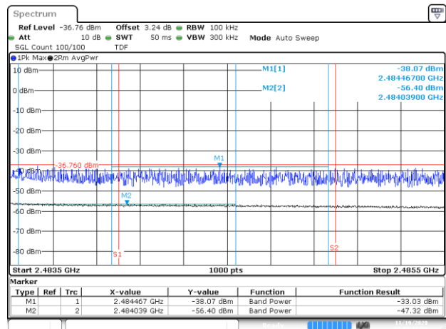
BE-R-HIGH-2MHz, DIV-2, 802.11ax20-HE0, Ch13
