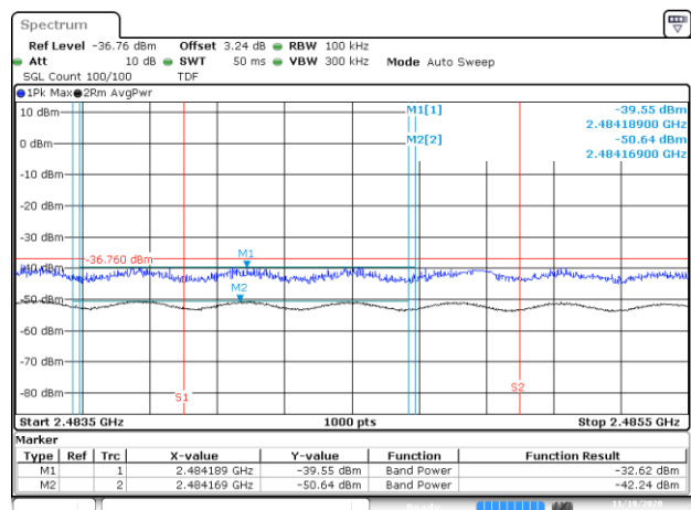
BE-R-HIGH-2MHz, DIV-2, 802.11n40-HT0, Ch10
