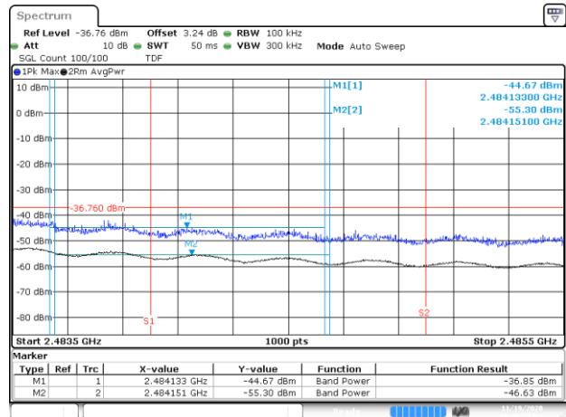
BE-R-HIGH-2MHz, DIV-2, 802.11g-6Mbps, Ch12
