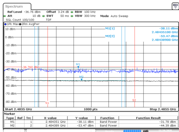
BE-R-HIGH-2MHz, DIV-2, 802.11ax40-HE0, Ch11
