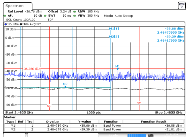
BE-R-HIGH-2MHz, DIV-2, 802.11g-6Mbps, Ch13
