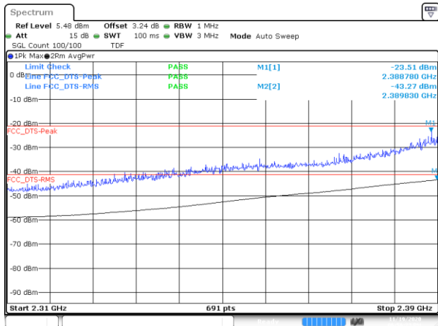
BE-R-LOW, DIV-2, 802.11n40-HT0, Ch3
