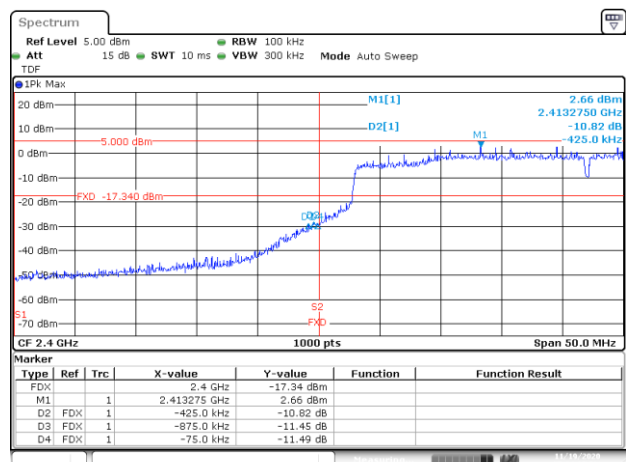
BE-NR, DIV-2, 802.11ax40-HE0, Ch3
