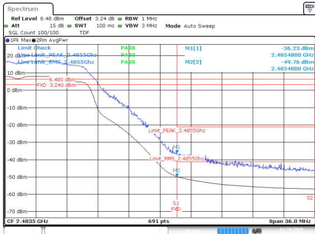
BE-R-HIGH, DIV-2, 802.11g-6Mbps, Ch12
