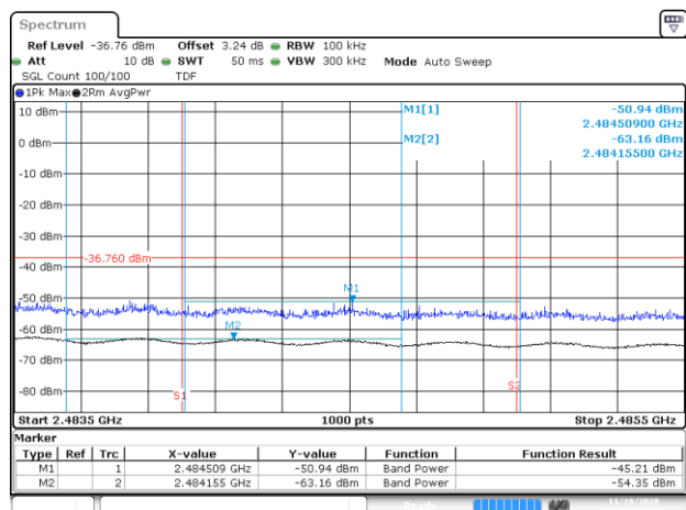
BE-R-HIGH-2MHz, DIV-2, 802.11g-6Mbps, Ch11
