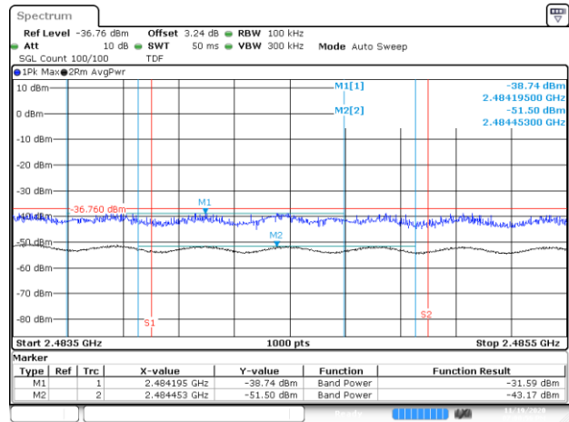
BE-R-HIGH-2MHz, DIV-2, 802.11n40-HT0, Ch11
