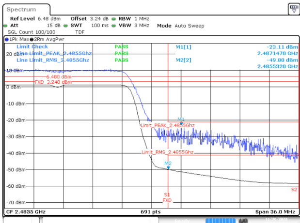
BE-R-HIGH, DIV-2, 802.11n20-HT0, Ch13
