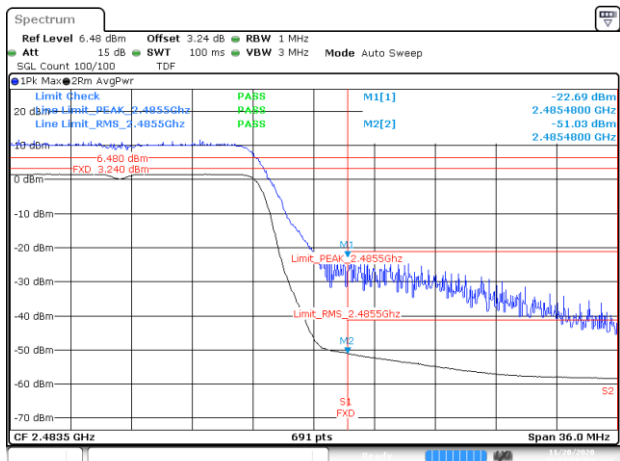
BE-R-HIGH, DIV-2, 802.11g-6Mbps, Ch13
