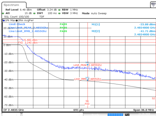
BE-R-HIGH, DIV-2, 802.11n40-HT0, Ch9
