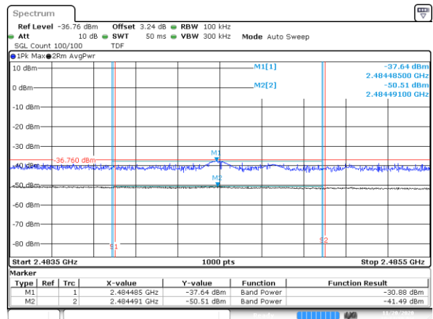
BE-R-HIGH-2MHz, DIV-2, 802.11ax40-HE0, Ch10
