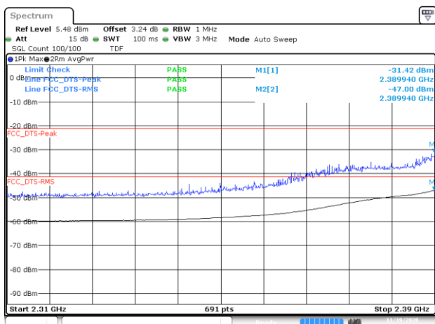
BE-R-LOW, DIV-2, 802.11n20-HT0, Ch1
