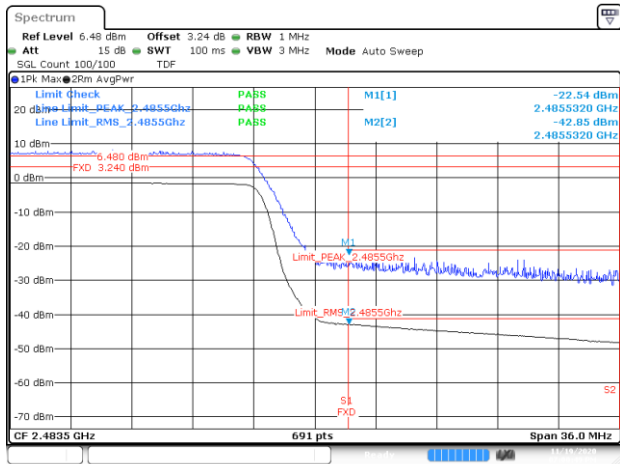
BE-R-HIGH, DIV-2, 802.11n40-HT0, Ch11
