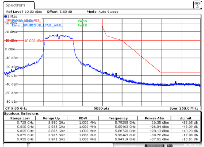
SISO A, 802.11n40, HT0, CH159, BE High Peak
