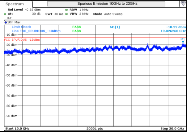
LTE 4 16QAM BW15MHz High Ch 20325 1RB-0
