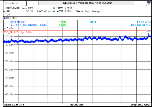
LTE 4 16QAM BW15MHz Low Ch 20025 1RB-0
