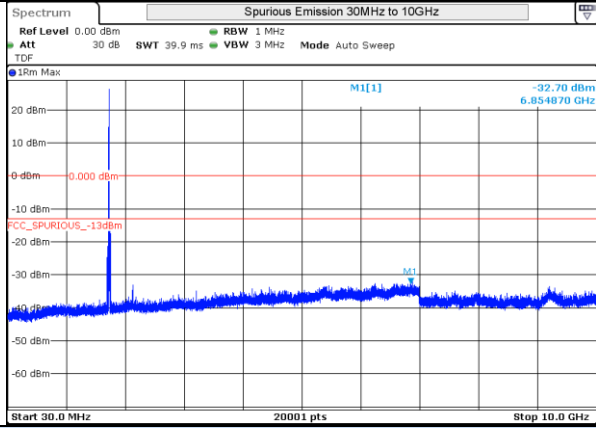
LTE 4 16QAM BW15MHz High Ch 20325 1RB-0
