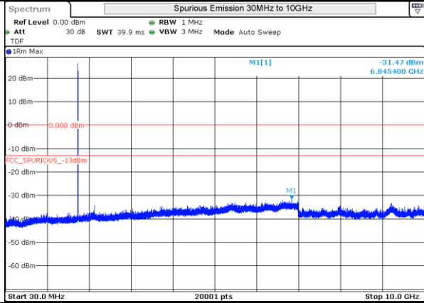
LTE 4 16QAM BW3MHz High Ch 20385 1RB-0
