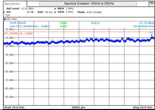
LTE 4 16QAM BW15MHz Mid Ch 20175 1RB-0
