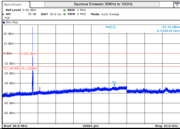
LTE 4 16QAM BW15MHz Mid Ch 20175 1RB-0
