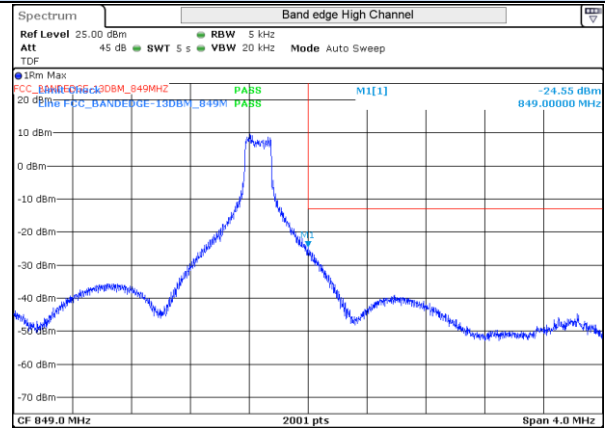
LTE 5 QPSK BW5MHz High channel 20625 1RB-24
