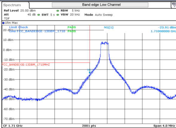
LTE 4 16QAM BW5MHz Low channel 19975 1RB-0
