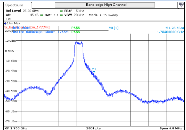
LTE 4 QPSK BW5MHz High channel 20375 1RB-24
