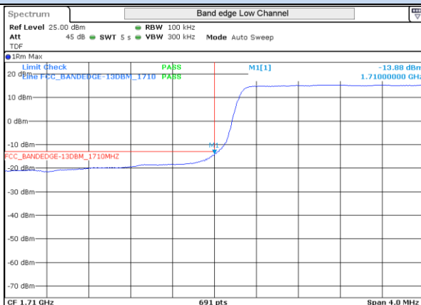
LTE 4 QPSK BW5MHz Low channel 19975 25RB-0
