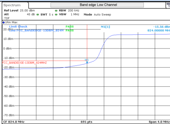
LTE 5 QPSK BW10MHz Low channel 20450 50RB-0
