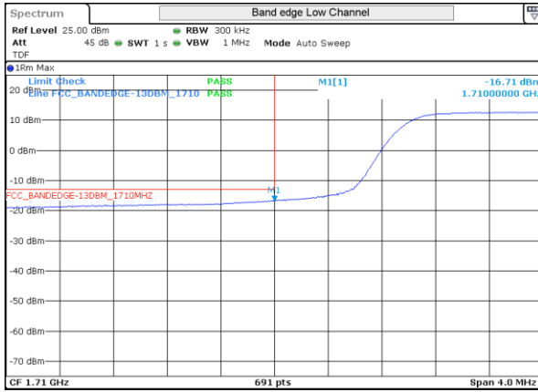
LTE 4 16QAM BW20MHz Low channel 20050 100RB-0
