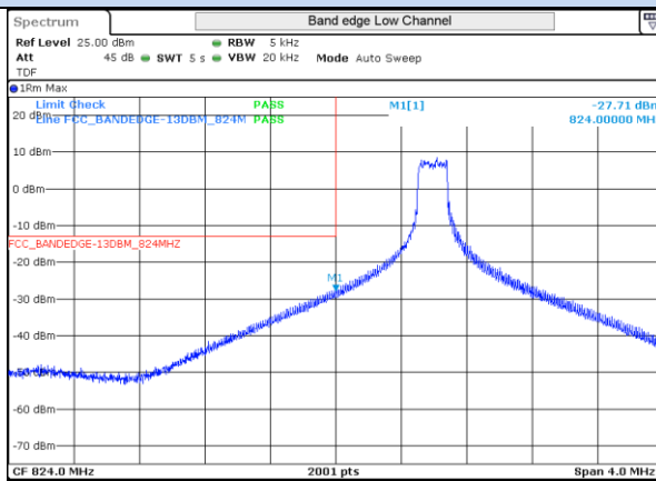
LTE 5 16QAM BW10MHz Low channel 20450 1RB-0
