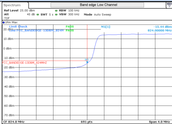
LTE 5 16QAM BW5MHz Low channel 20425 1RB-0
