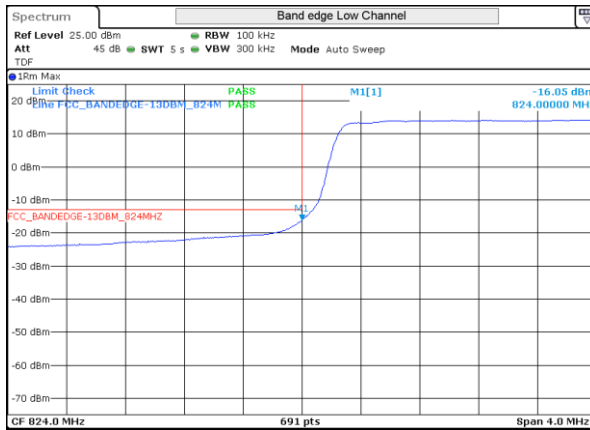
LTE 5 16QAM BW5MHz Low channel 20425 25RB-0
