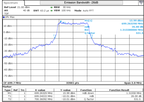
LTE 12 16QAM BW1.4MHz 699.7MHz Low ch 23017 6RB-0
