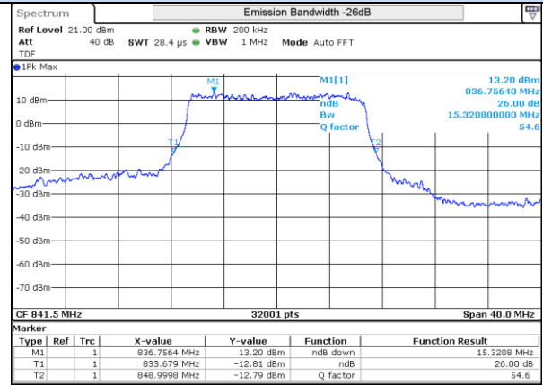
LTE 26 16QAM BW15MHz 841.5MHz High ch 26965 75RB-0
