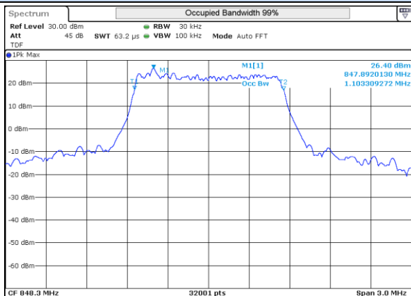
LTE 26 16QAM BW1.4MHz 848.3MHz High ch 27033 6RB-0
