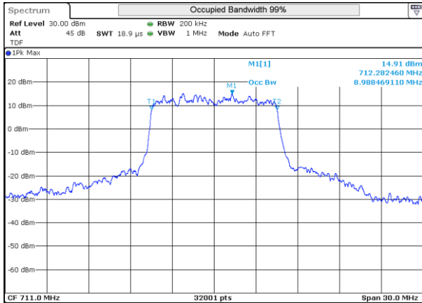
LTE 12 16QAM BW10MHz 711MHz High ch 23130 50RB-0
