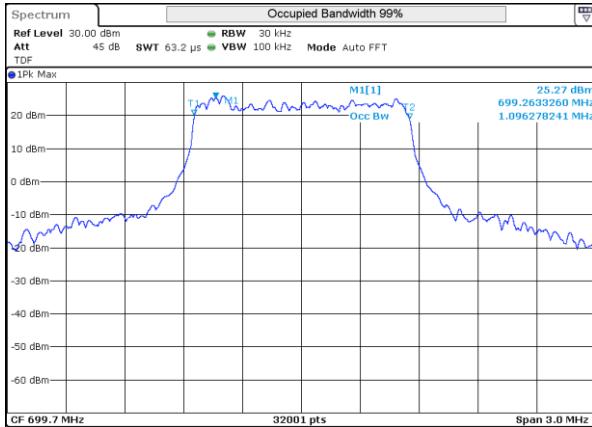
LTE 12 16QAM BW1.4MHz 699.7MHz Low ch 23017 6RB-0
