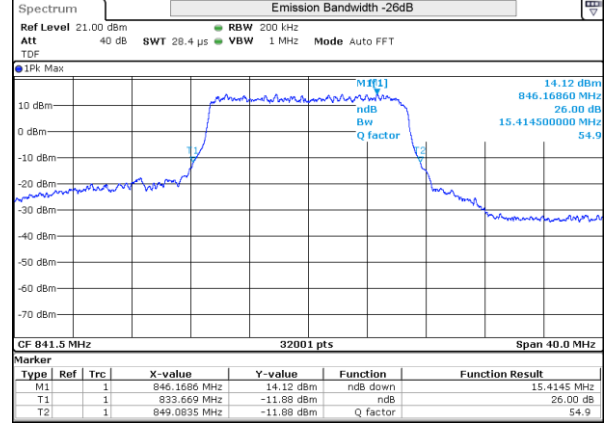
LTE 26 QPSK BW15MHz 841.5MHz High ch 26965 75RB-0
