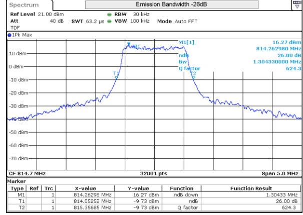
LTE 26 16QAM BW1.4MHz 814.7MHz Low ch 26697 6RB-0
