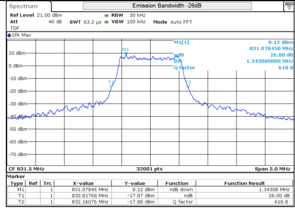
LTE 26 16QAM BW1.4MHz 831.5MHz Mid ch 26865 6RB-0
