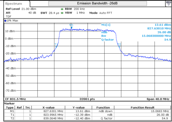
LTE 26 16QAM BW15MHz 831.5MHz Mid ch 26865 75RB-0
