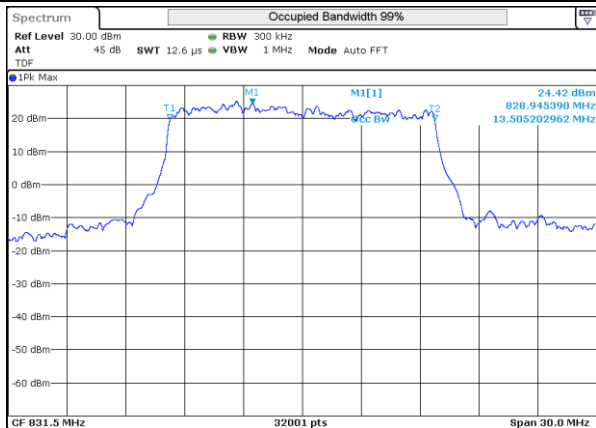
LTE 26 16QAM BW15MHz 831.5MHz Mid ch 26865 75RB-0
