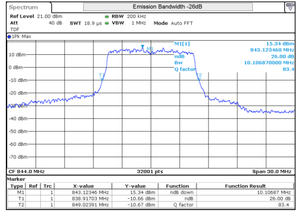
LTE 26 16QAM BW10MHz 844MHz High ch 26990 50RB-0
