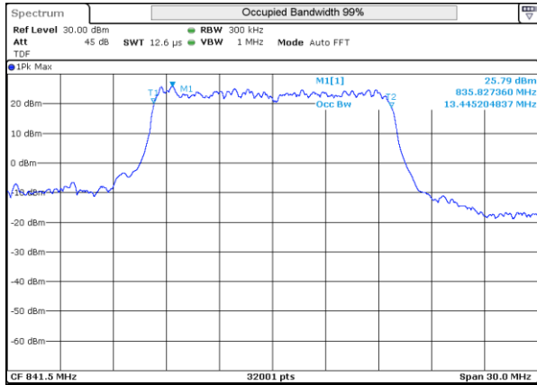
LTE 26 QPSK BW15MHz 841.5MHz High ch 26965 75RB-0
