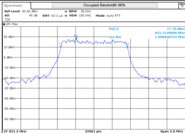
LTE 26 16QAM BW1.4MHz 831.5MHz Mid ch 26865 6RB-0
