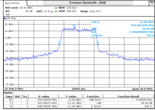
LTE 26 16QAM BW5MHz 846.5MHz High ch 27015 25RB-0
