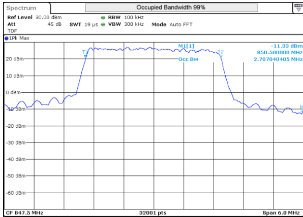
LTE 26 16QAM BW3MHz 847.5MHz High ch 27025 15RB-0
