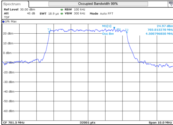
LTE 12 16QAM BW3MHz 701.5MHz High ch 23035 25RB-0
