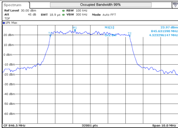
LTE 26 16QAM BW5MHz 846.5MHz High ch 27015 25RB-0
