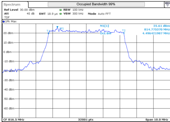
LTE 26 16QAM BW5MHz 816.5MHz Low ch 26715 25RB-0
