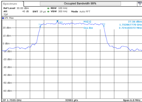
LTE 4 16QAM BW3MHz High ch 20385 15RB-0
