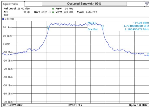
LTE 4 16QAM BW1.4MHz Mid ch 20175 6RB-0
