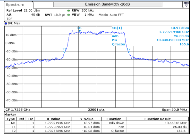
LTE 4 16QAM BW10MHz Mid ch 20175 50RB-0
