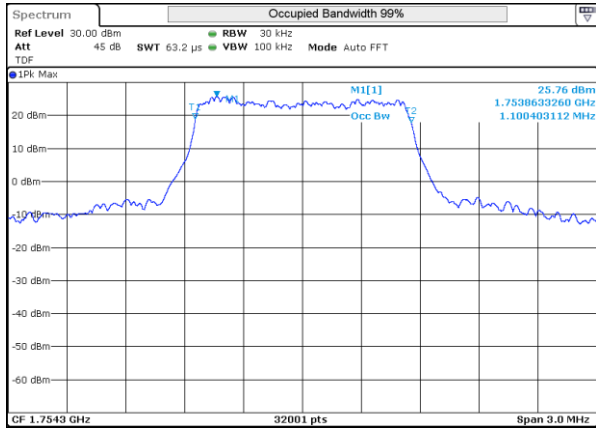
LTE 4 16QAM BW1.4MHz High ch 20393 6RB-0
