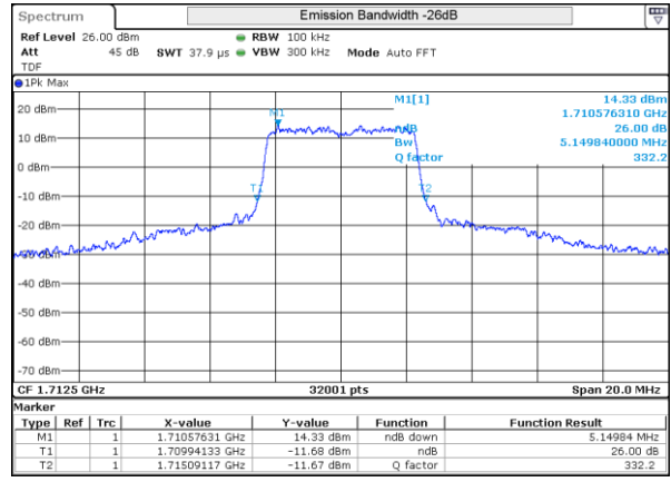
LTE 4 16QAM BW5MHz Low ch 19975 25RB-0
