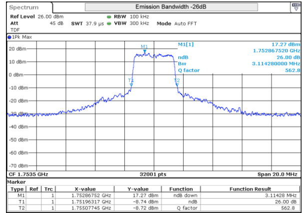
LTE 4 16QAM BW3MHz High ch 20385 15RB-0
