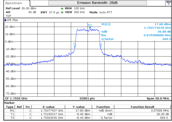
LTE 4 QPSK BW3MHz High ch 20385 15RB-0
