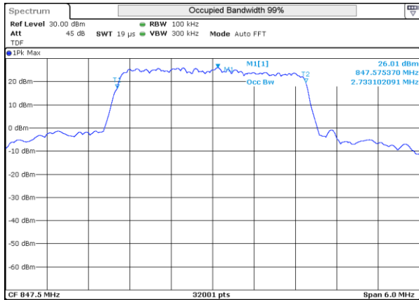
LTE 5 16QAM BW3MHz High ch 20635 15RB-0
