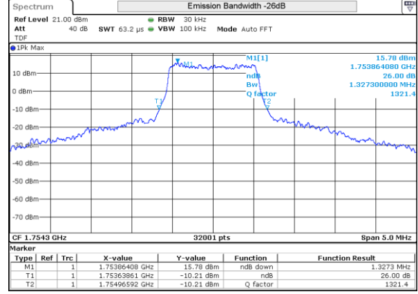
LTE 4 16QAM BW1.4MHz High ch 20393 6RB-0
