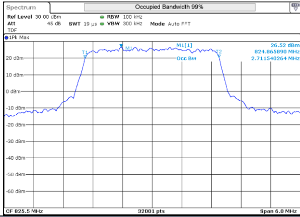
LTE 5 16QAM BW3MHz Low ch 20415 15RB-0
