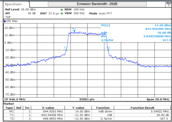
LTE 5 16QAM BW5MHz High ch 20625 25RB-0
