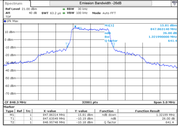
LTE 5 16QAM BW1.4MHz High ch 20643 6RB-0
