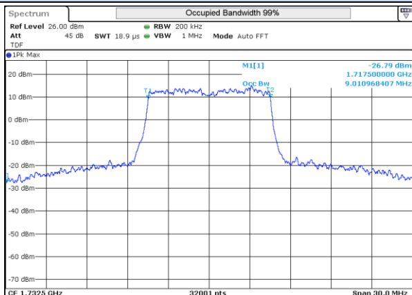
LTE 4 16QAM BW10MHz Mid ch 20175 50RB-0
