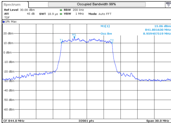
LTE 5 16QAM BW10MHz High ch 20600 50RB-0
