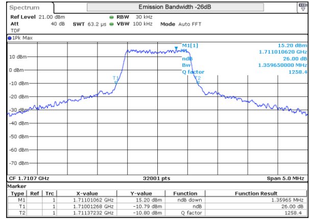
LTE 4 16QAM BW1.4MHz Low ch 19957 6RB-0
