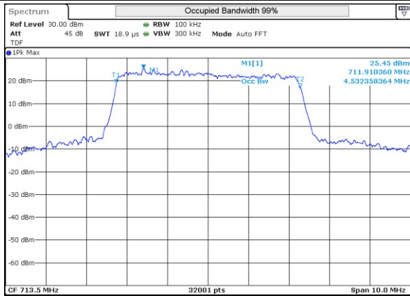
LTE 17 16QAM BW5MHz High ch 23825 25RB-0
