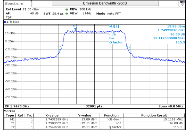
LTE 4 16QAM BW15MHz Mid ch 20175 75RB-0
