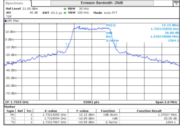
LTE 4 16QAM BW1.4MHz Mid ch 20175 6RB-0
