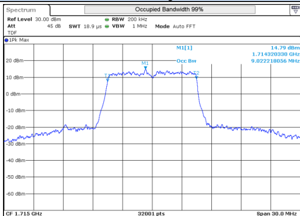
LTE 4 16QAM BW10MHz Low ch 20000 50RB-0
