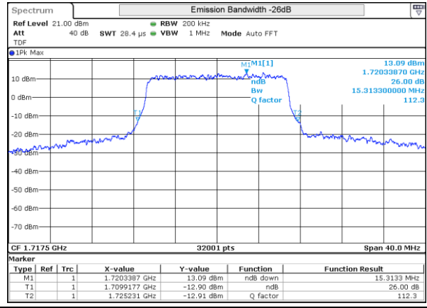
LTE 4 16QAM BW15MHz Low ch 20025 75RB-0
