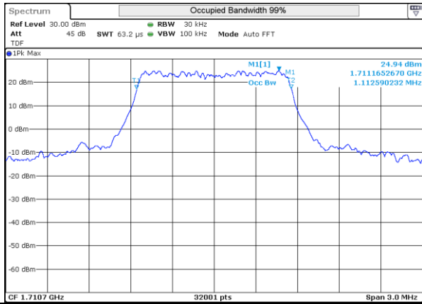
LTE 4 16QAM BW1.4MHz Low ch 19957 6RB-0
