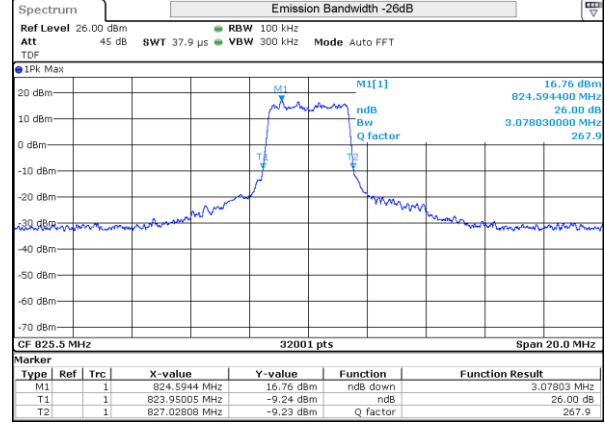
LTE 5 16QAM BW3MHz Low ch 20415 15RB-0
