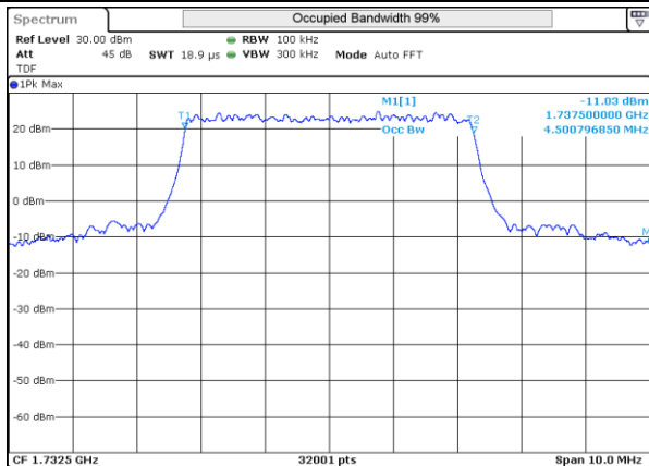
LTE 4 16QAM BW5MHz Mid ch 1975 25RB-0
