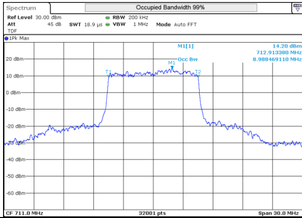
LTE 17 16QAM BW10MHz High ch 23800 50RB-0
