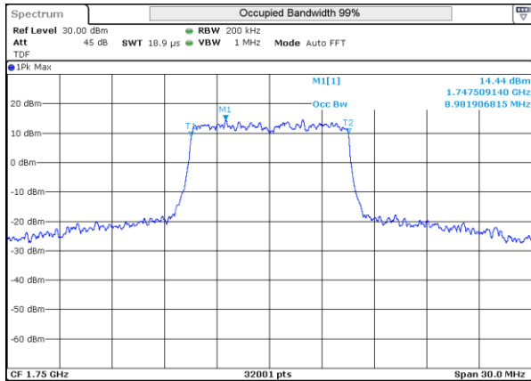
LTE 4 16QAM BW10MHz High ch 20350 50RB-0
