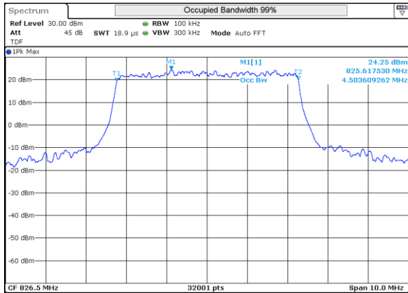
LTE 5 16QAM BW5MHz Low ch 20425 25RB-0
