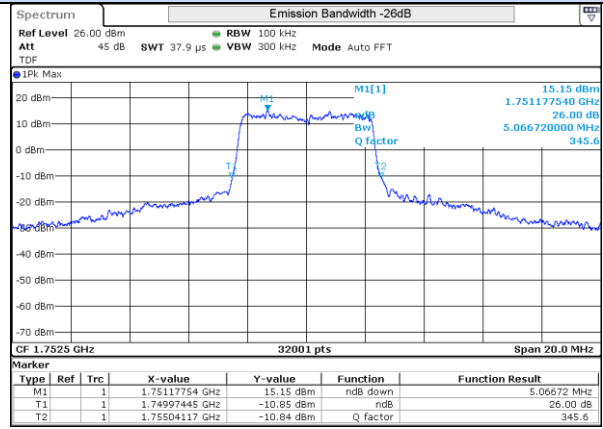
LTE 4 16QAM BW5MHz High ch 20175 25RB-0
