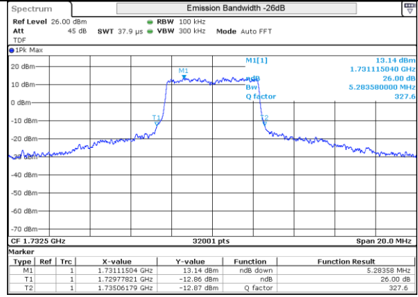
LTE 4 16QAM BW5MHz Mid ch 1975 25RB-0
