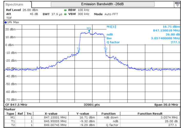
LTE 5 16QAM BW3MHz High ch 20635 15RB-0
