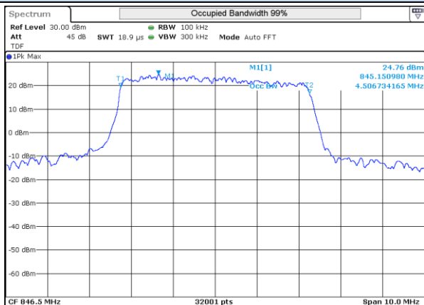
LTE 5 16QAM BW5MHz High ch 20625 25RB-0
