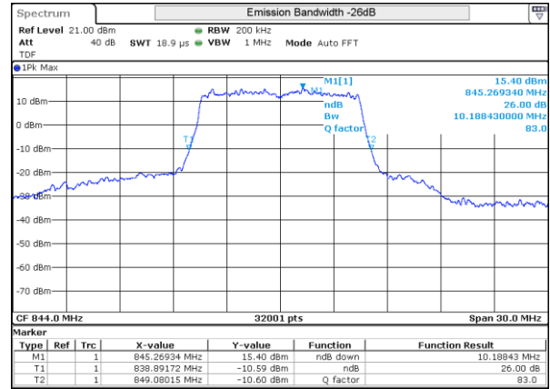
LTE 5 16QAM BW10MHz High ch 20600 50RB-0
