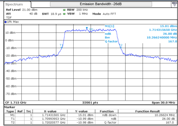
LTE 4 16QAM BW10MHz Low ch 20000 50RB-0
