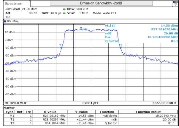
LTE 5 16QAM BW10MHz Low ch 20450 50RB-0
