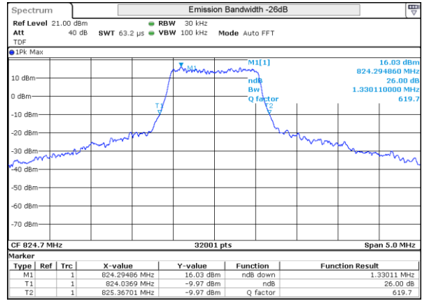
LTE 5 16QAM BW1.4MHz Low ch 20407 6RB-0
