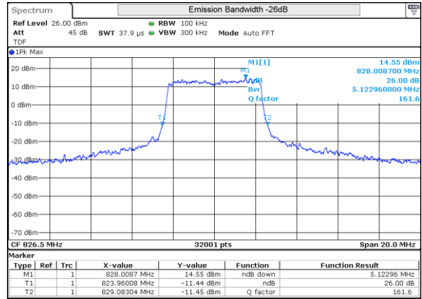
LTE 5 16QAM BW5MHz Low ch 20425 25RB-0
