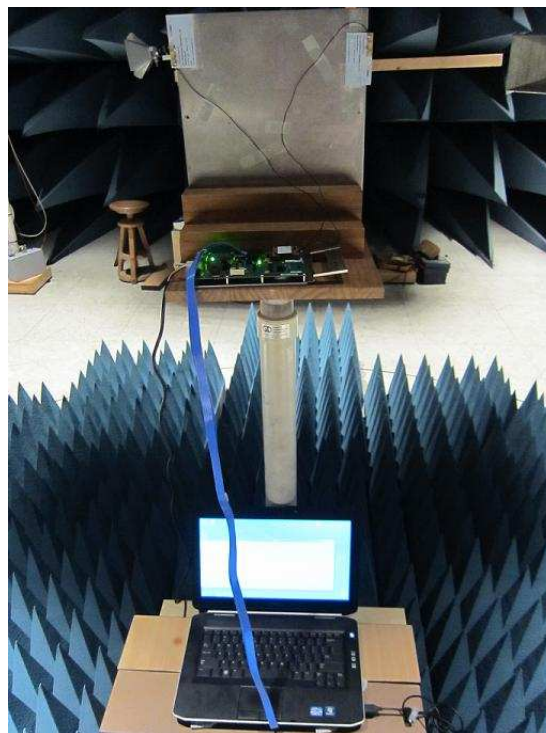
Fig. 3. Antenna frontal view
