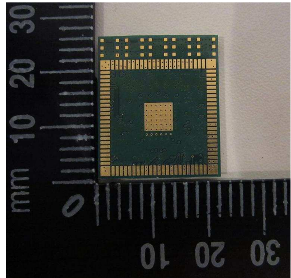
Fig. 2. Module rear view
