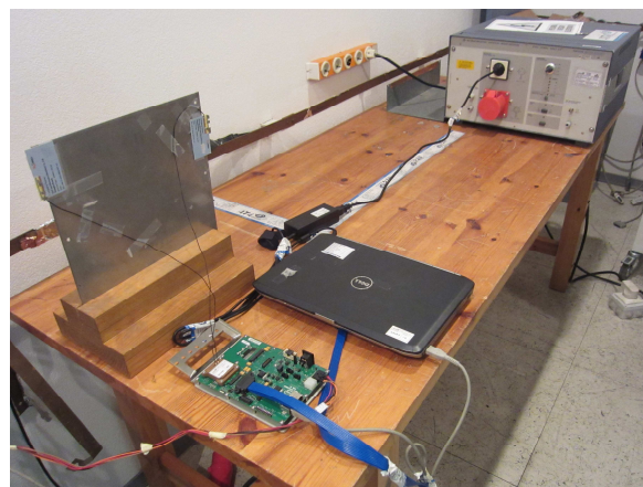
Fig. 7. Test set-up for conducted measurements
