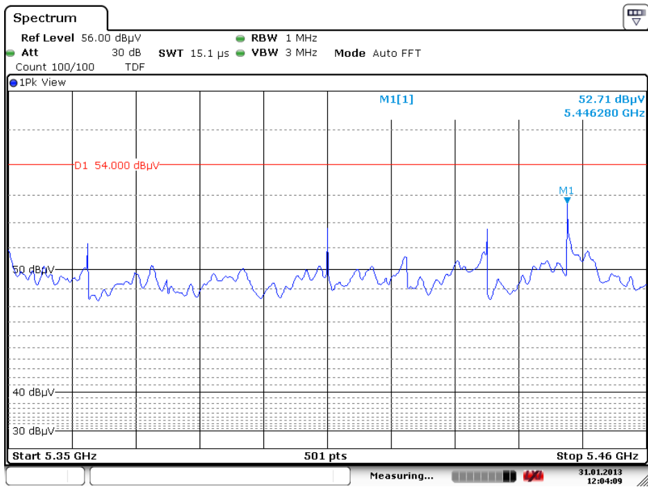
Emissions in restricted band 5.35-5.46 GHz, Average value, 6Mb OFDM, 5240 MHz valid for Antenna 2
