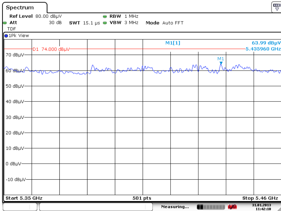
Emissions in restricted band 5.35-5.46 GHz, Peak value, 6Mb OFDM, 5240 MHz valid for Antenna 2
