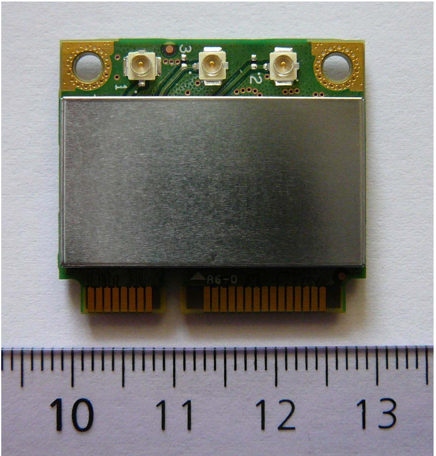
Top View “Insulation removed”
