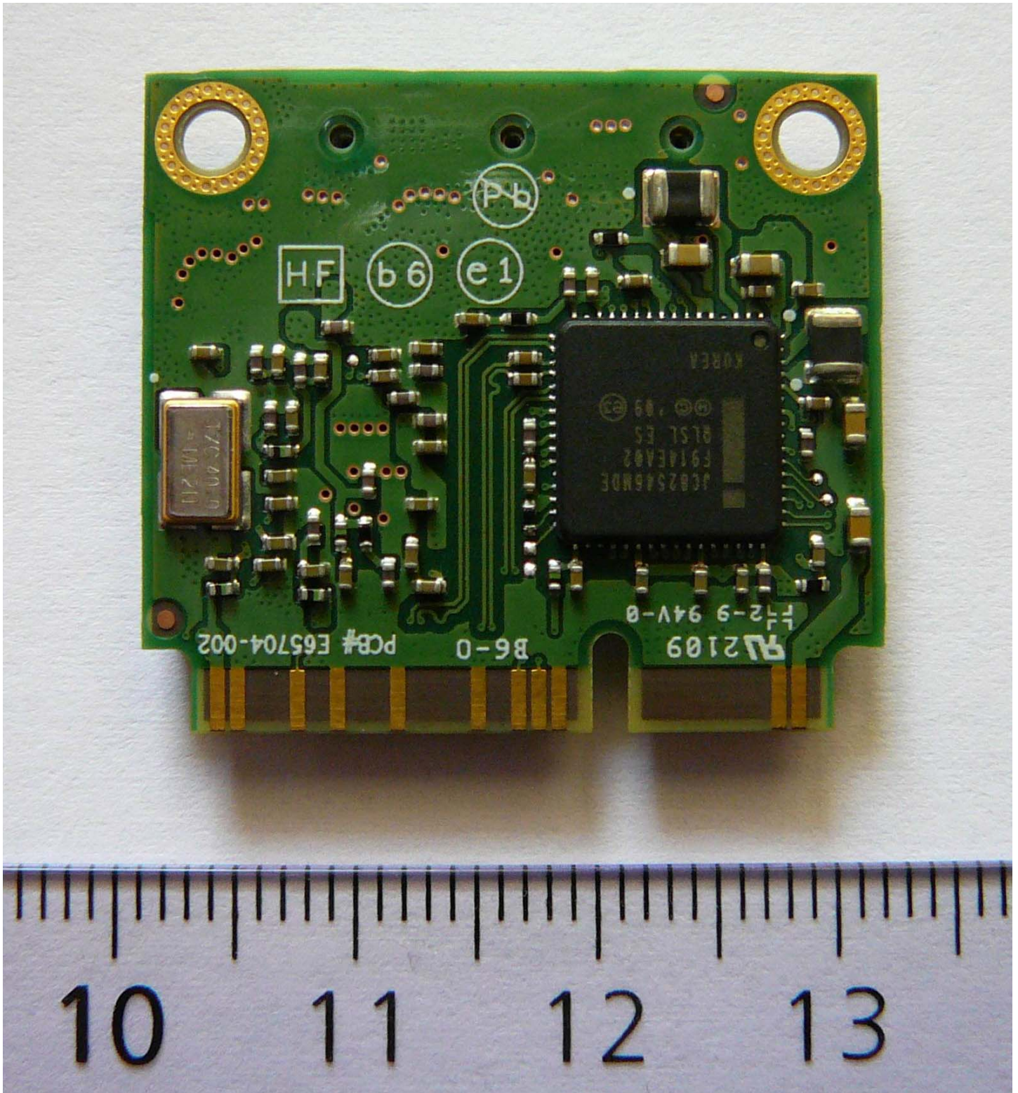
Bottom View “Insulation removed”
