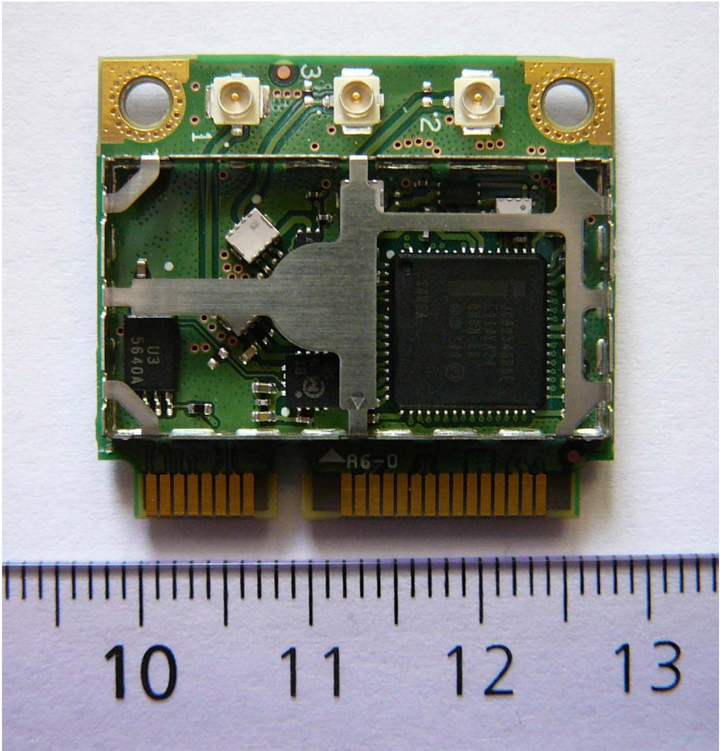
Top View “Shielding removed”
