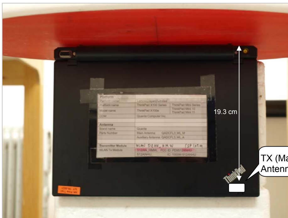
Setup photo for Routine SAR Evaluation
