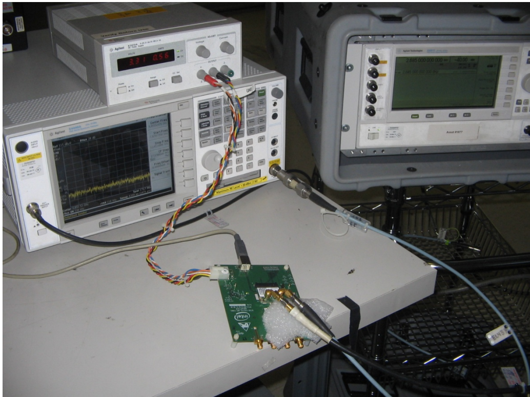
Test configuration, Radiated Emissions (Top) and Antenna Port Measurements (Bottom)
