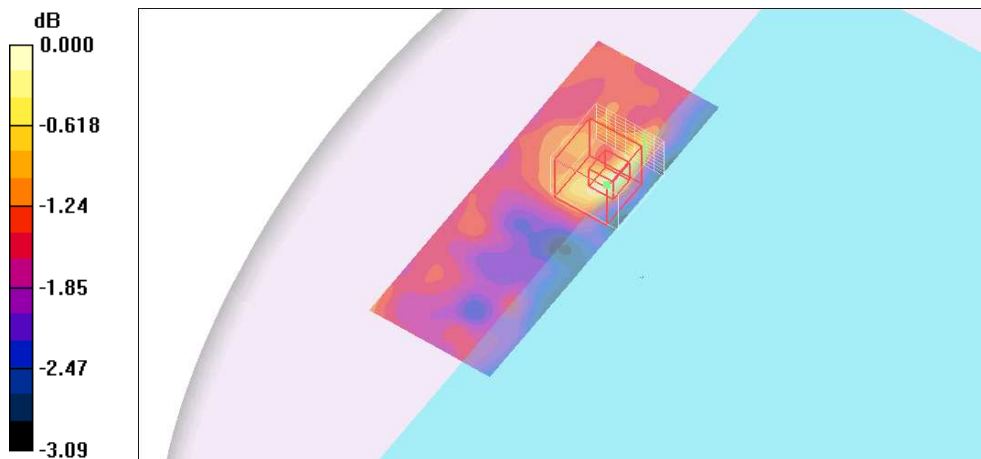
0 dB = 0.097mW/g
