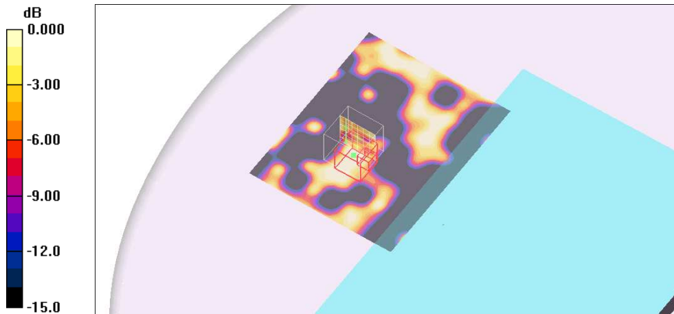
0 dB = 0.002mW/g
