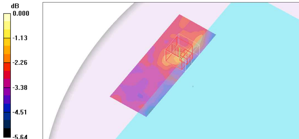
0 dB = 0.132mW/g
