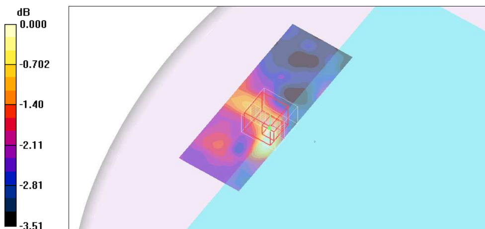
0 dB = 0.140mW/g
