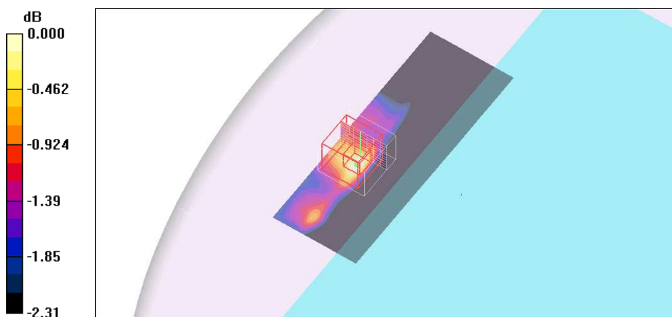
0 dB = 0.126mW/g
