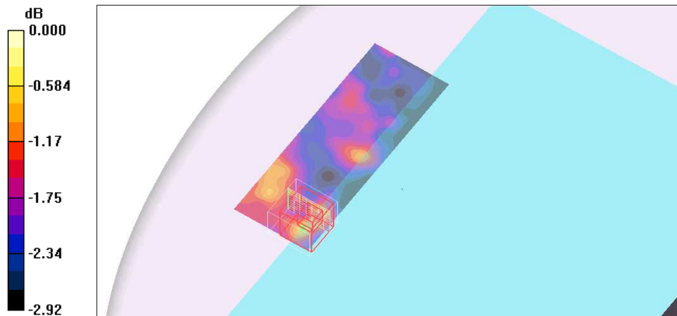
0 dB = 0.097mW/g
