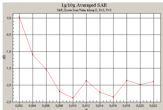
0 dB = 0.137mW/g
