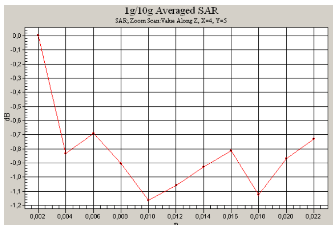
0 dB = 0.126mW/g
