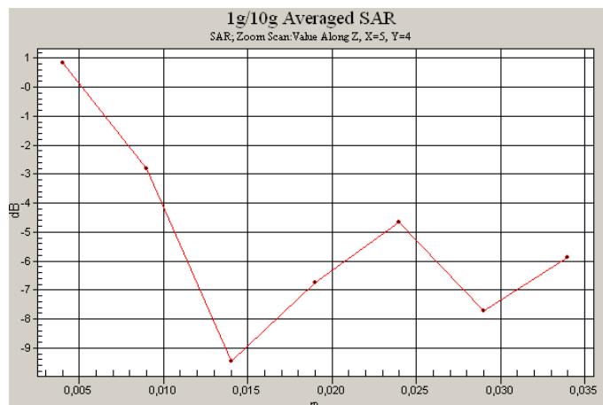
0 dB = 0.002mW/g
