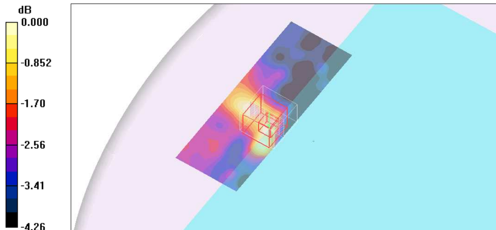
0 dB = 0.137mW/g
