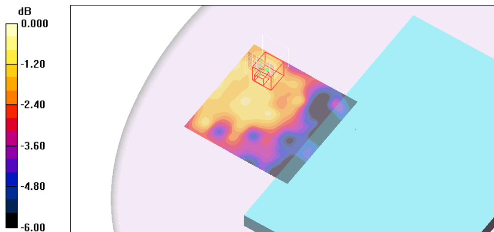
0 dB = 0.006mW/g
