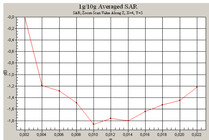
0 dB = 0.135mW/g
