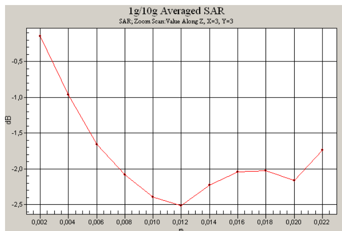
0 dB = 0.140mW/g
