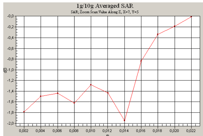
0 dB = 0.097mW/g
