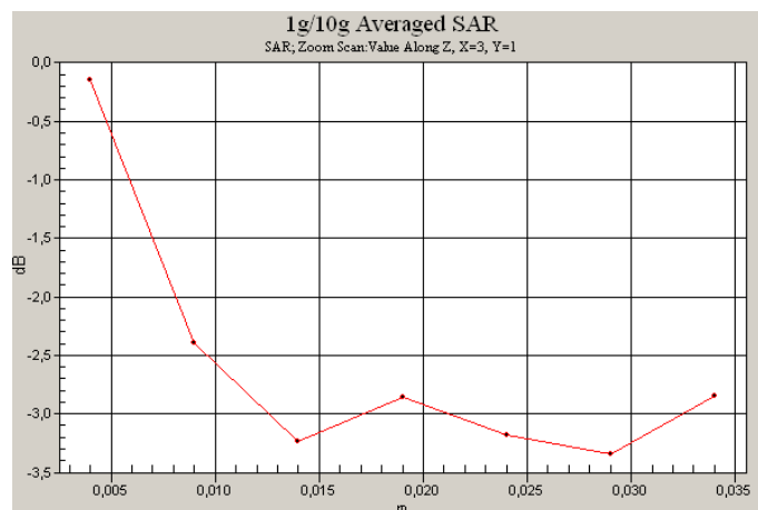
0 dB = 0.006mW/g
