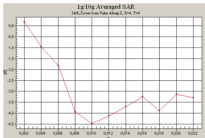
0 dB = 0.087mW/g
