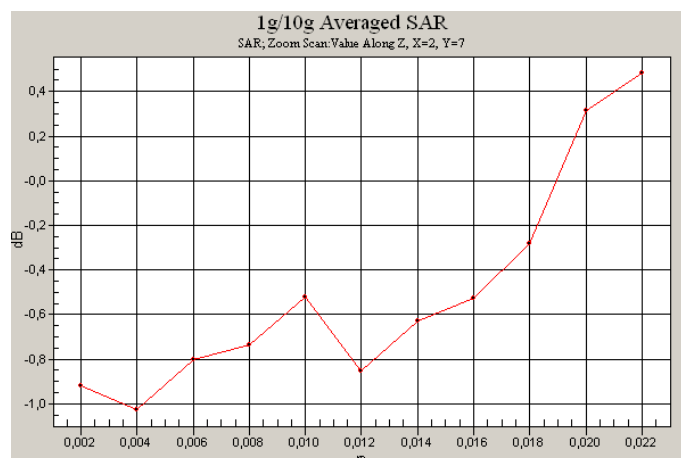
0 dB = 0.097mW/g
