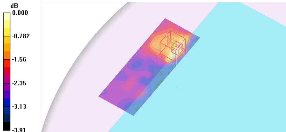
0 dB = 0.135mW/g
