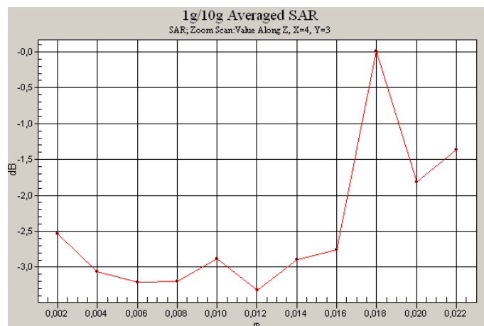
0 dB = 0.132mW/g
