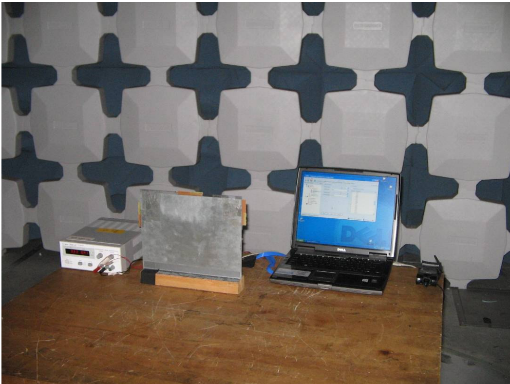
Radiated Emissions
