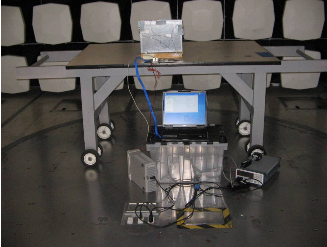
Radiated Emissions
