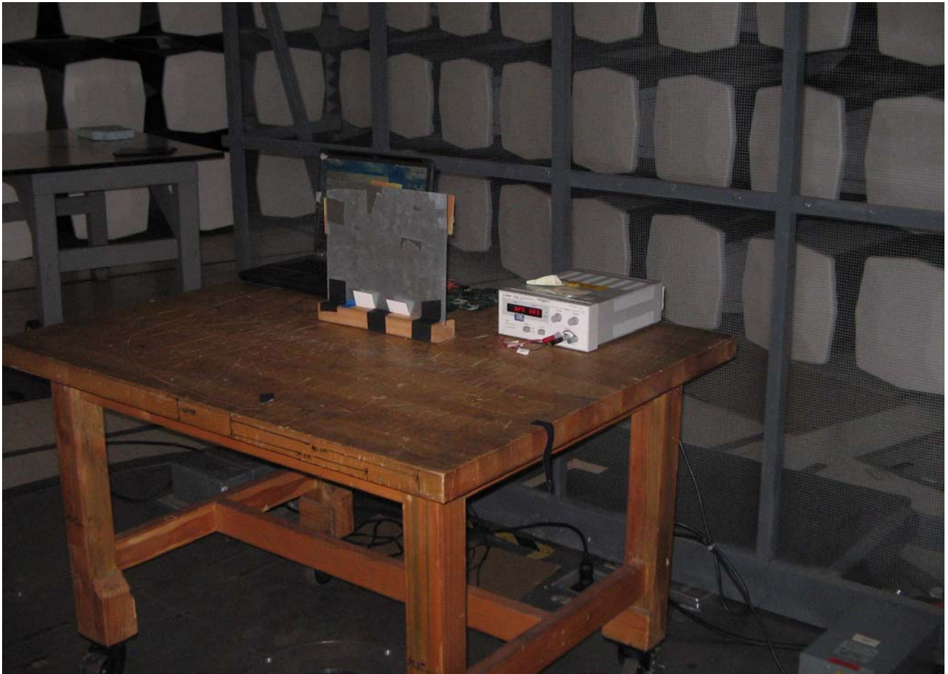
AC Conducted Emissions
