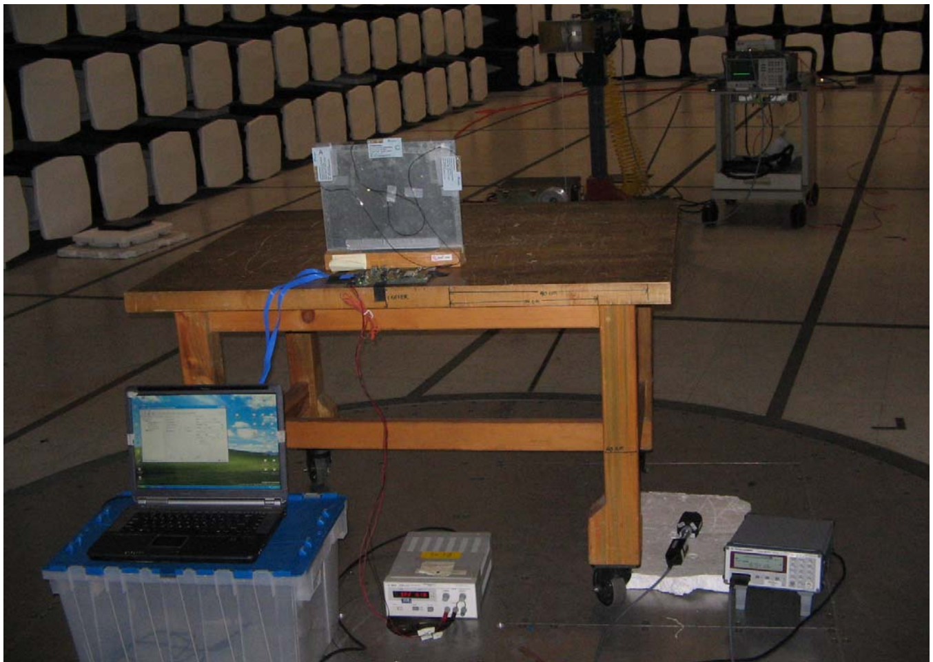
Radiated Emissions Configuration
