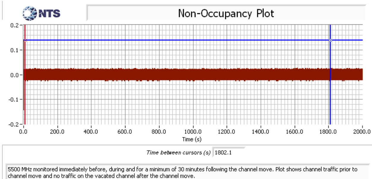
Figure 7 Radar Channel Non-Occupancy Plot, n20 Mode
