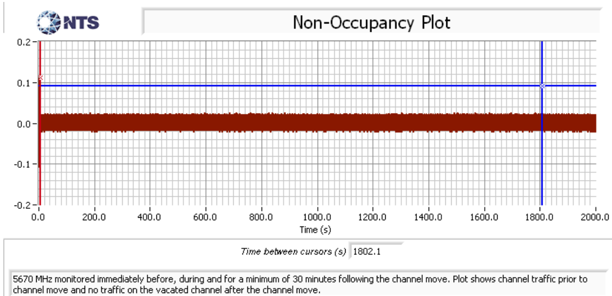
Figure 6 Radar Channel Non-Occupancy Plot, n40 Mode
