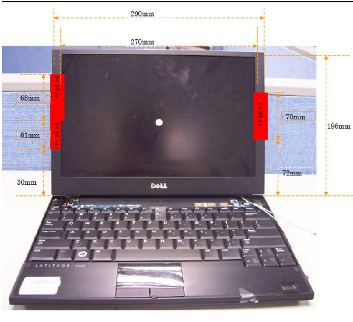
Antenna Locations WLAN (no RSB)
