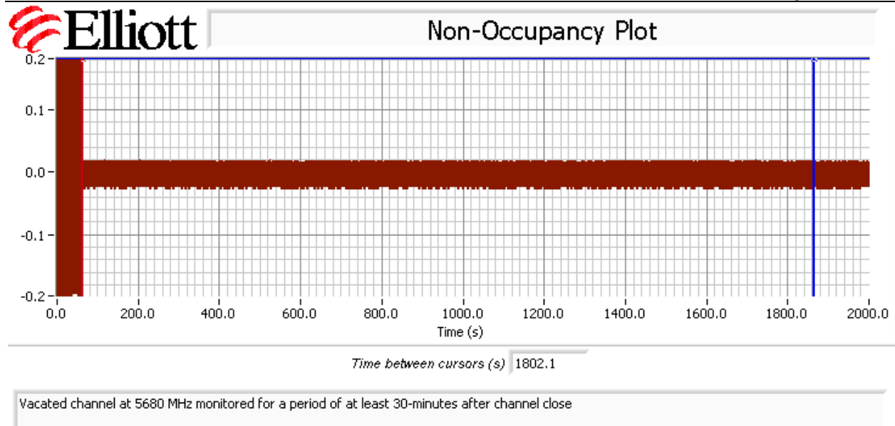
Figure 6 Radar Channel Non-Occupancy Plot (Associated Test)
