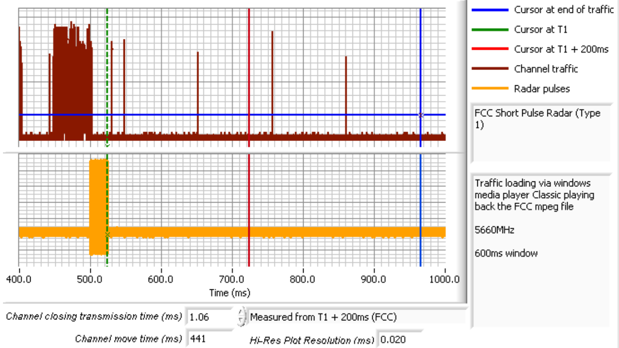
Figure 3 Close-Up of Transmissions Occurring More Than 200ms After The End of Radar, 20MHz BW
