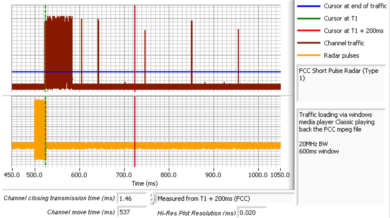
Figure 4 Close-Up of Transmissions Occurring More Than 200ms After The End of Radar (20MHz BW)
