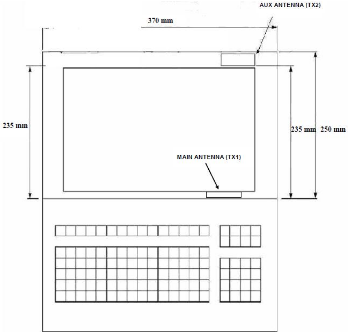
Antenna Locations
