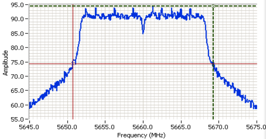
20 dB BW plots for closest channel to 5650 MHz
