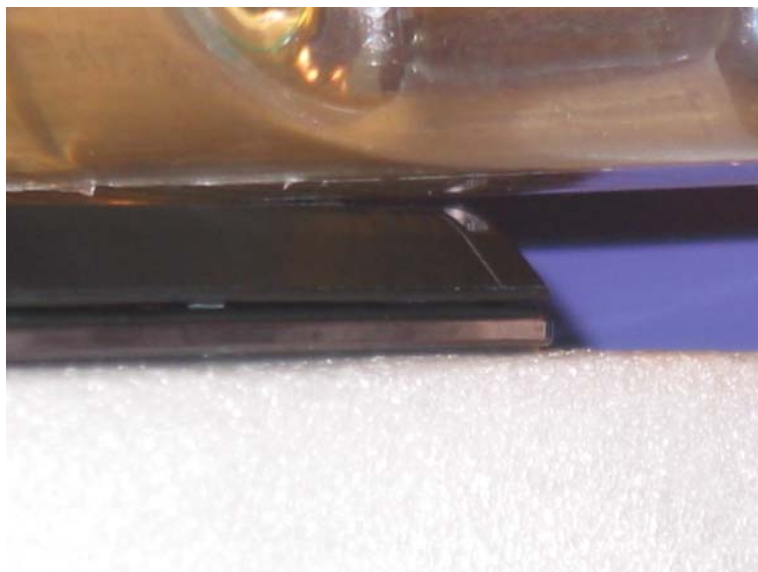
Test Position Side D Aux Antenna 0 mm Gap
