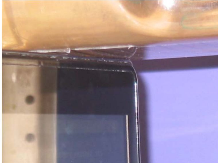
Test Position Side B Aux Antenna 0 mm Gap
