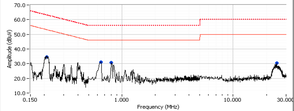
Run #1 230V/50Hz Neutral
