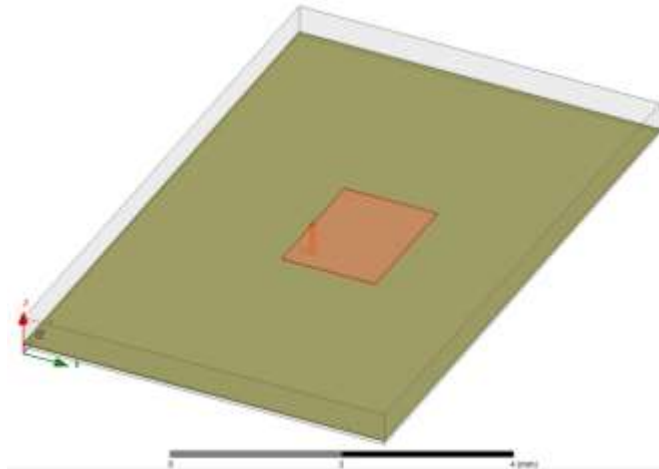
Figure 50 – Simulation of a single Patch antenna
