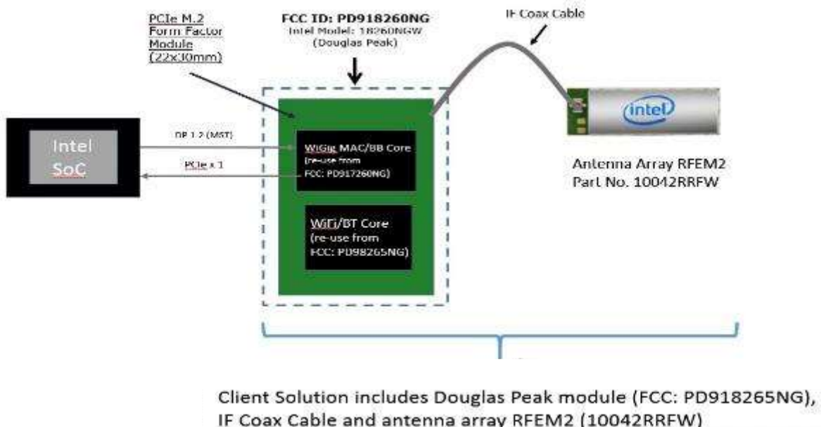
Figure 1 – Intel 18260NGW module system block diagram
