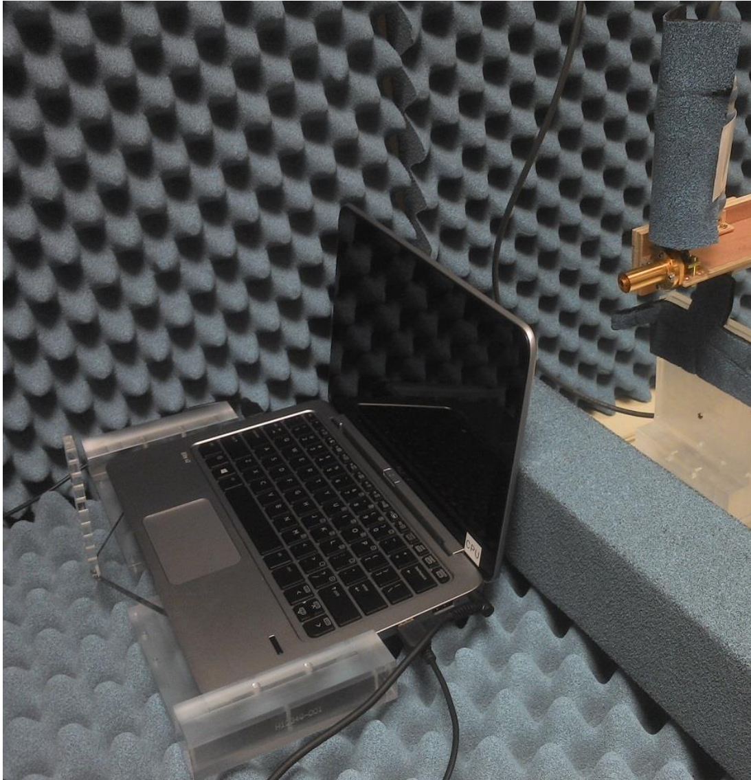
Figure 3 – Measurement Setup, Intel Regulatory Lab
