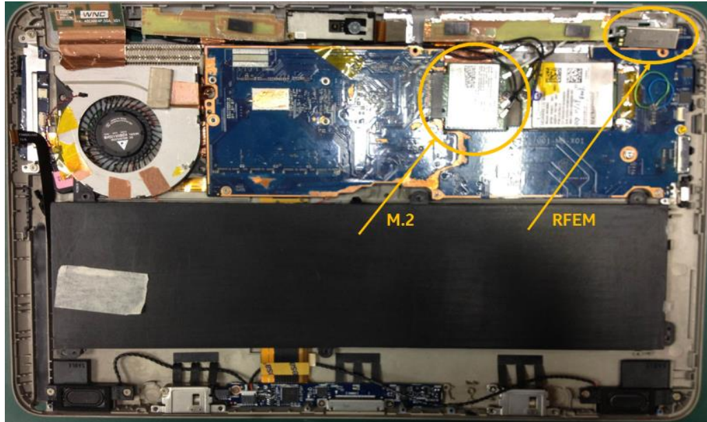
Figure 1 - Intel 17265NGW LC module inside HP PC model HSTNN-I22C platform
