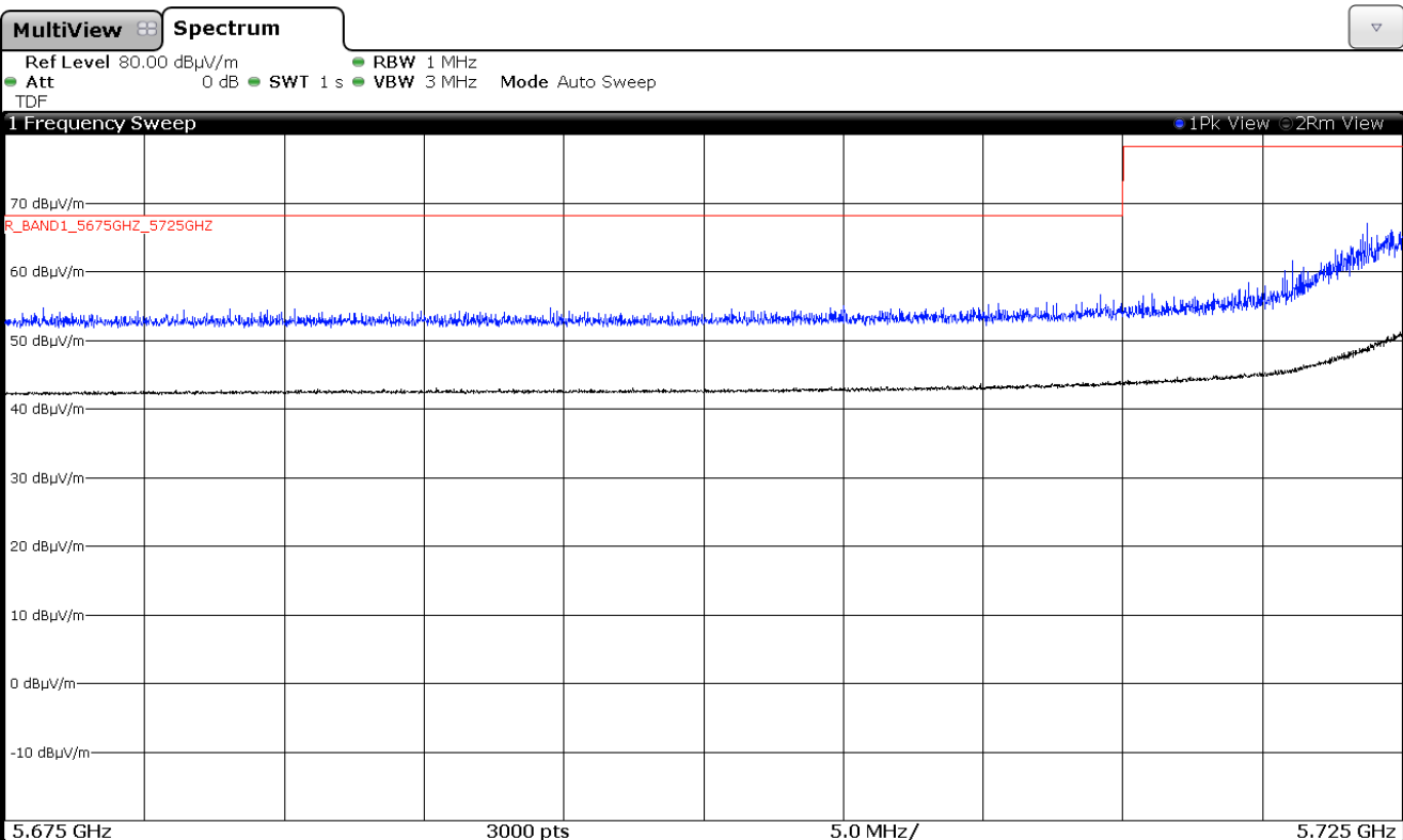
Chain B
