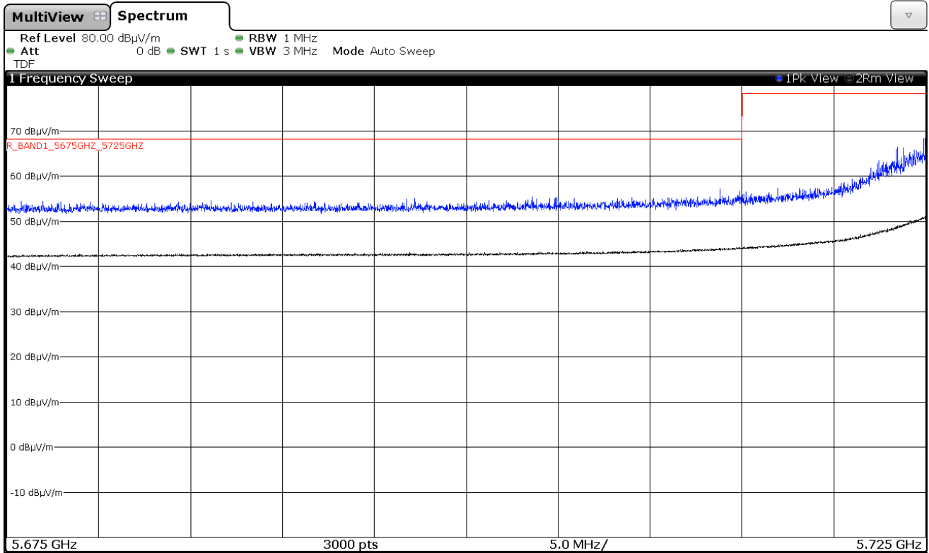
Chain A
