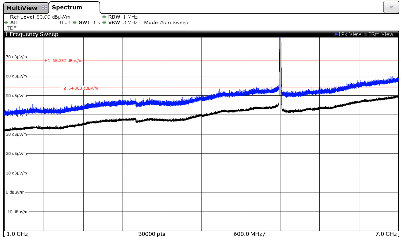
The peak above the limit is the carrier frequency. This plot is valid for both Chain A and Chain B.
