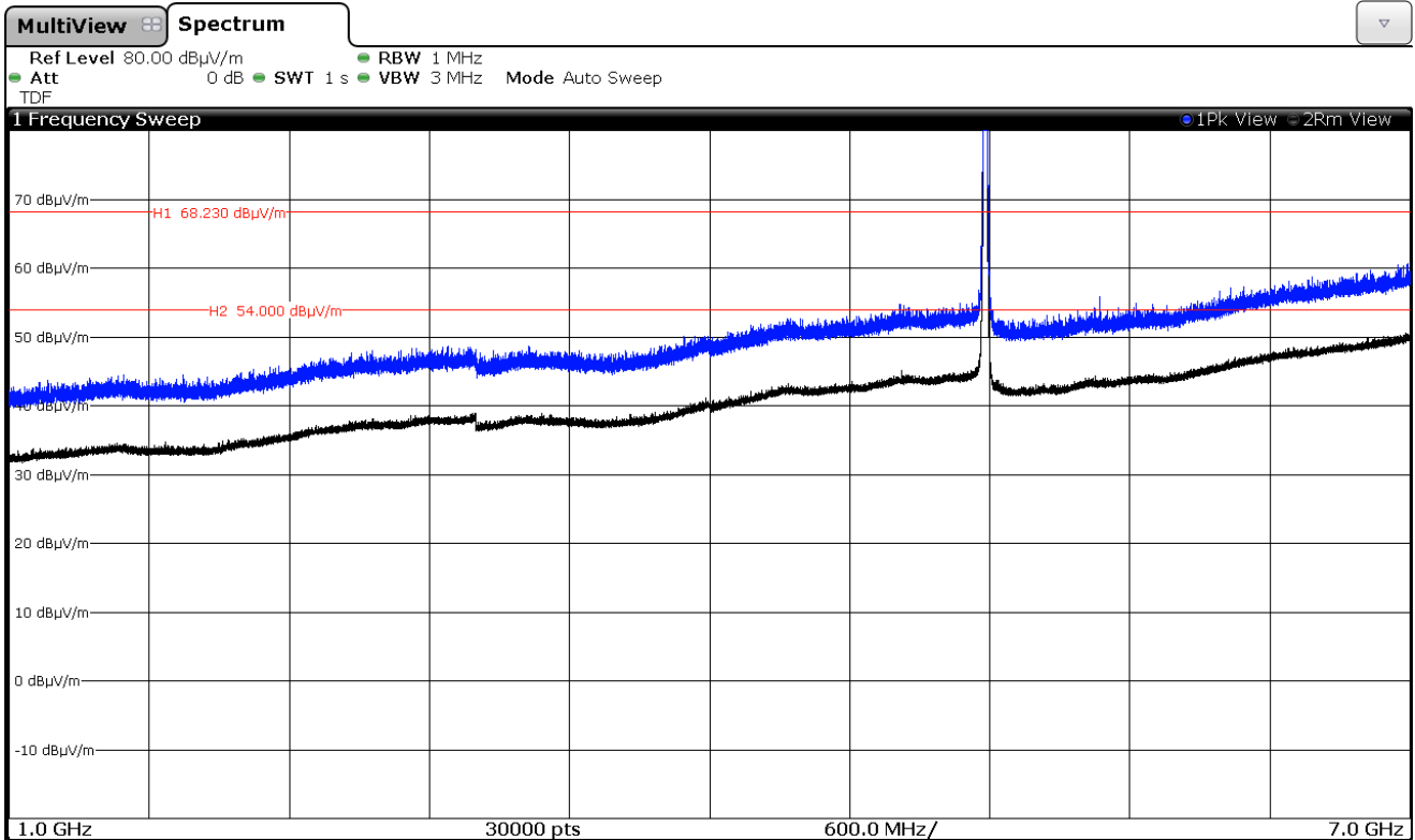
The peak above the limit is the carrier frequency. This plot is valid for both Chain A and Chain B.
