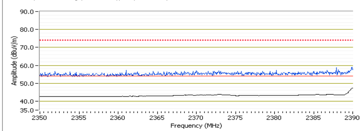
RB 1 MHz; VB 10 Hz Avg (Black Trace); PK (Blue Trace) Horizontal
