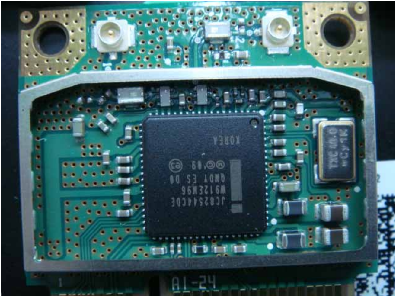
Close up of top side with shield removed
