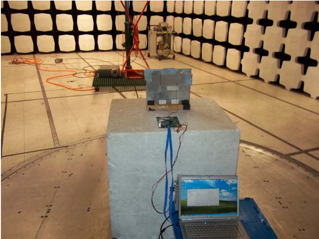
Radiated Emissions Test Configuration Photograph
