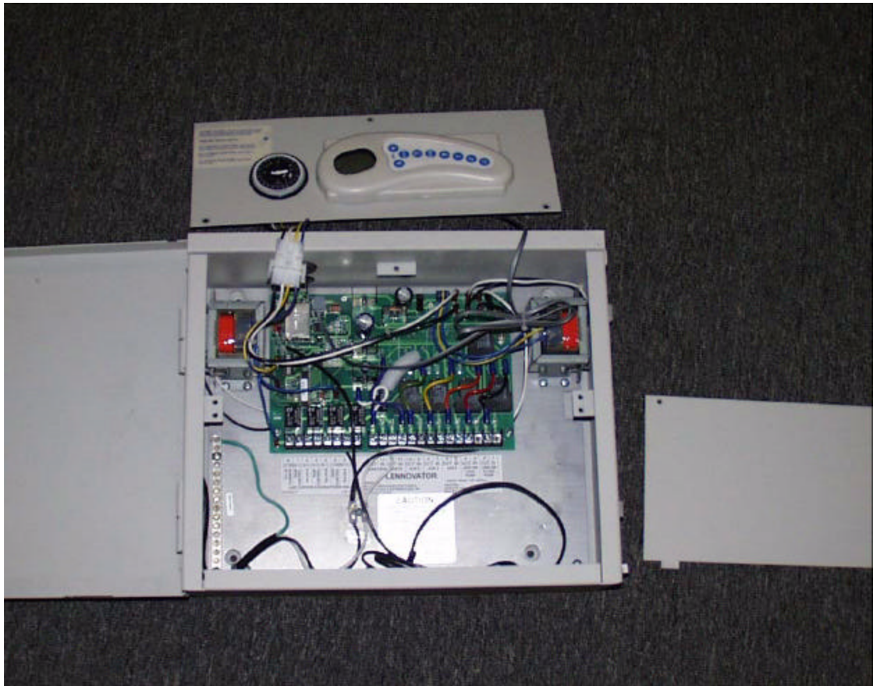
Inside Front Chassis
