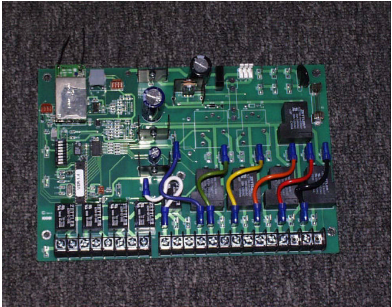
Control Board, Component Side
