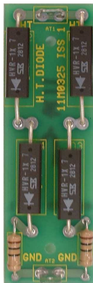
H.T. Diode Board Solder Side
