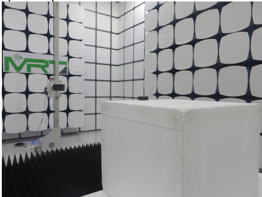
Photograph 3: Set-up for Radiated Test above 1GHz
