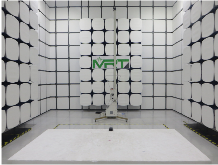
Photograph 2: Set-up for Radiated Test from 30MHz to 1GHz
