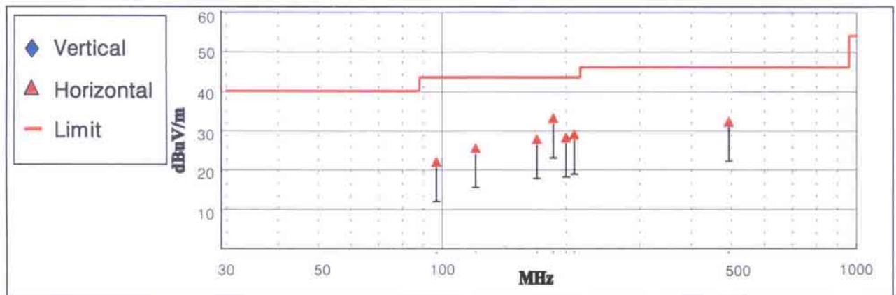
Fig 5. Graph of Radiated emission – Playing mode
