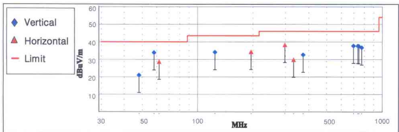
Fig 4. Graph of Radiated emission – Download mode
