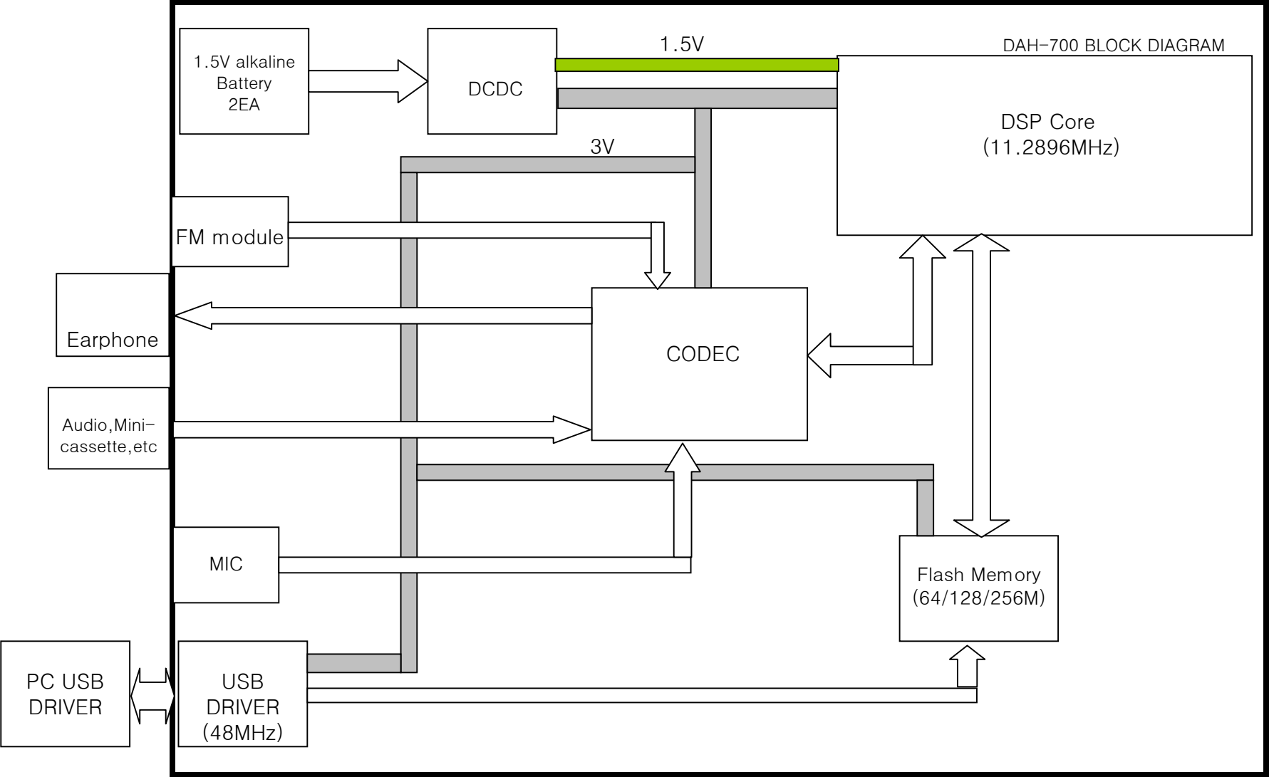
DAH-700 BLOCK DIAGRAM
