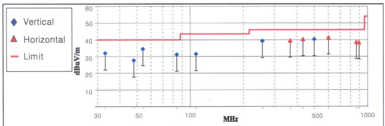
< Fig 6-1. Radiated emission result >
