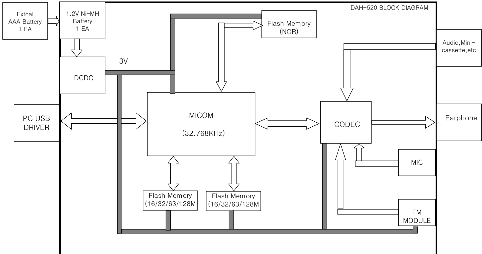
DAH-520 BLOCK DIAGRAM
