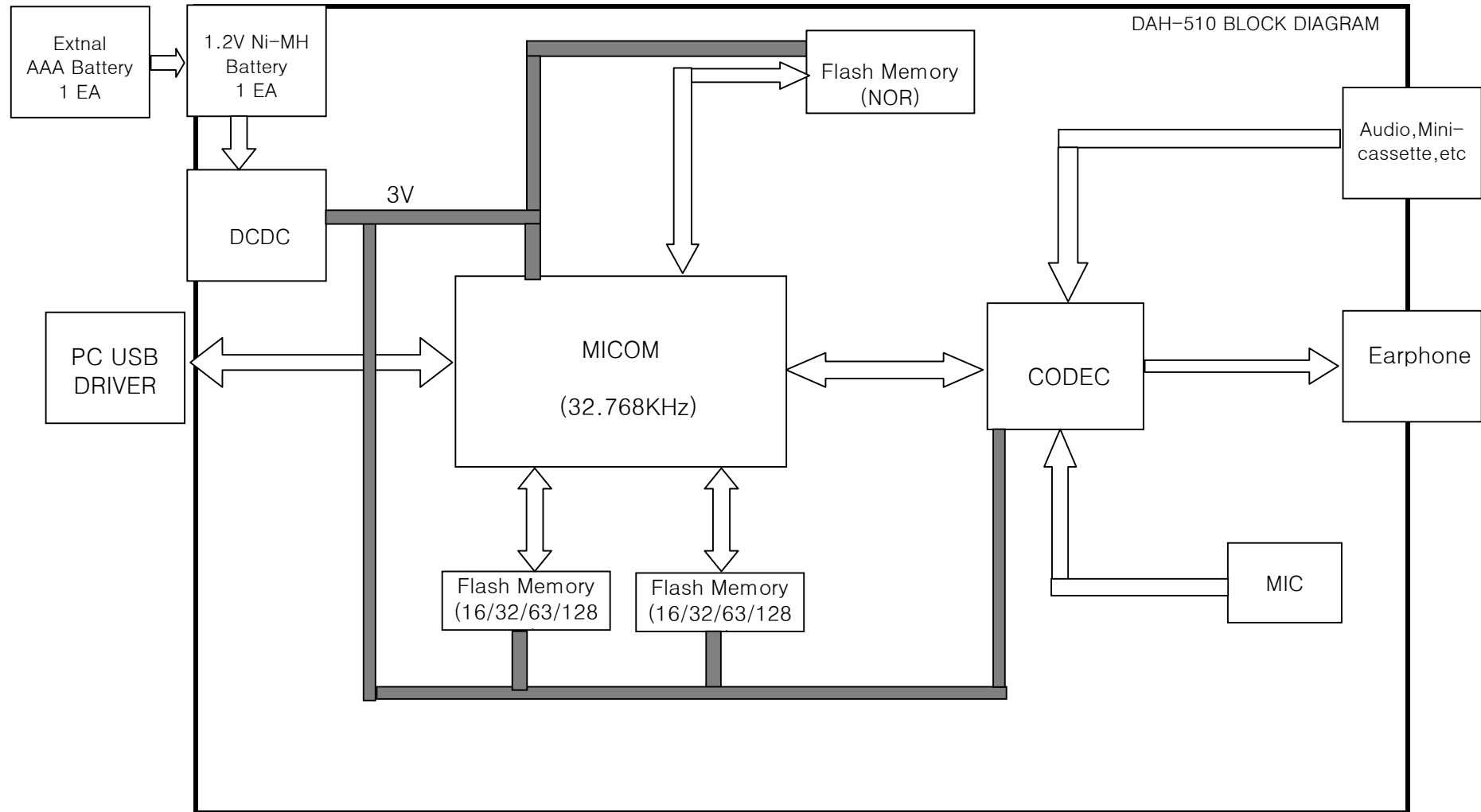
DAH-510 BLOCK DIAGRAM
