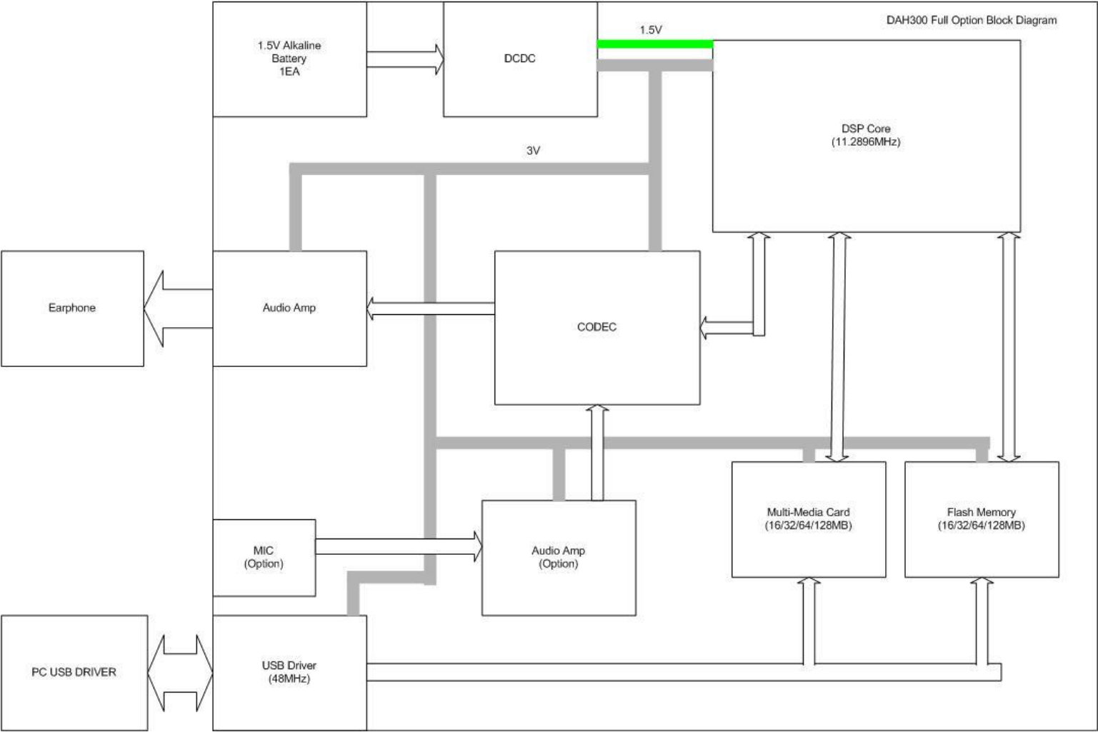
DAH300 Block Diagram
