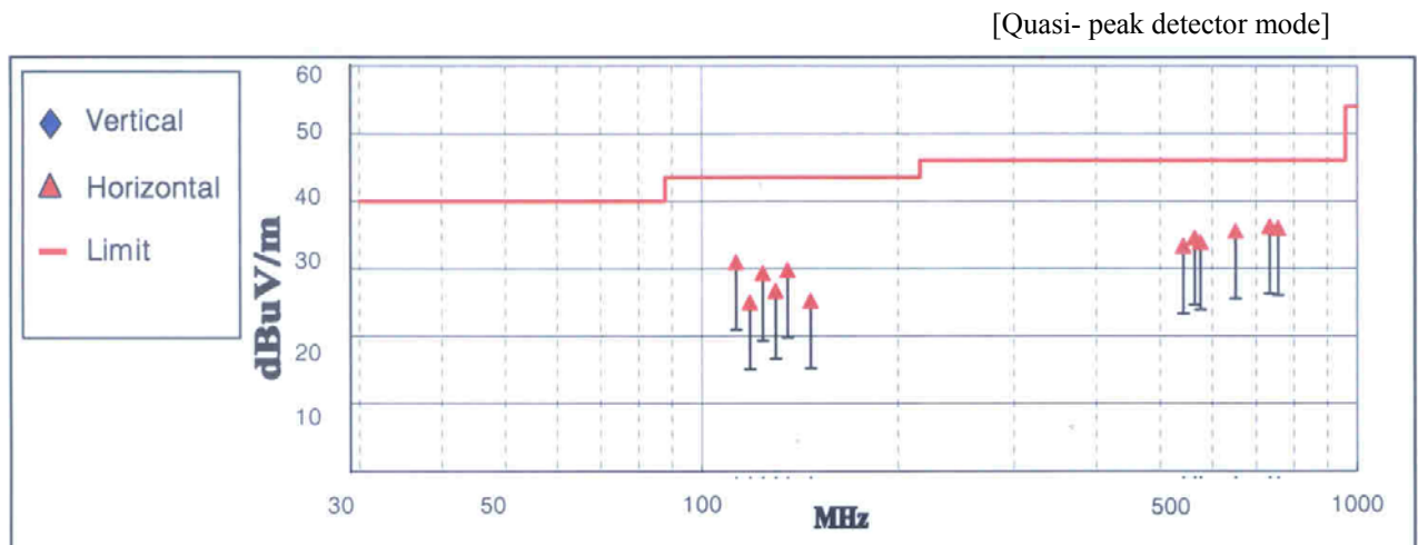
Fig 5. Graph of Radiated emission – Playing mode
