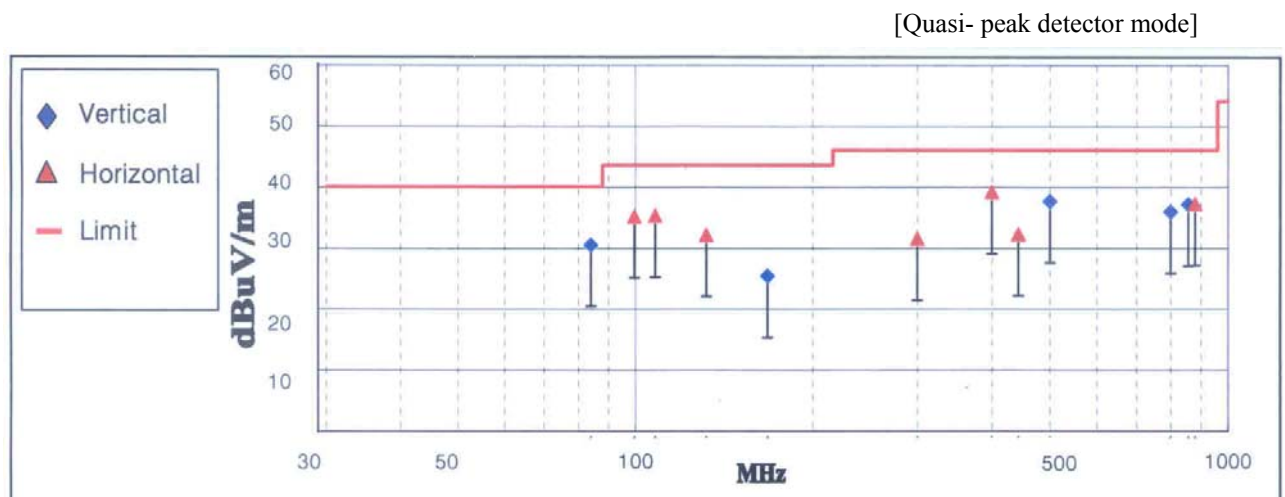
Fig 4. Graph of Radiated emission – Download mode
