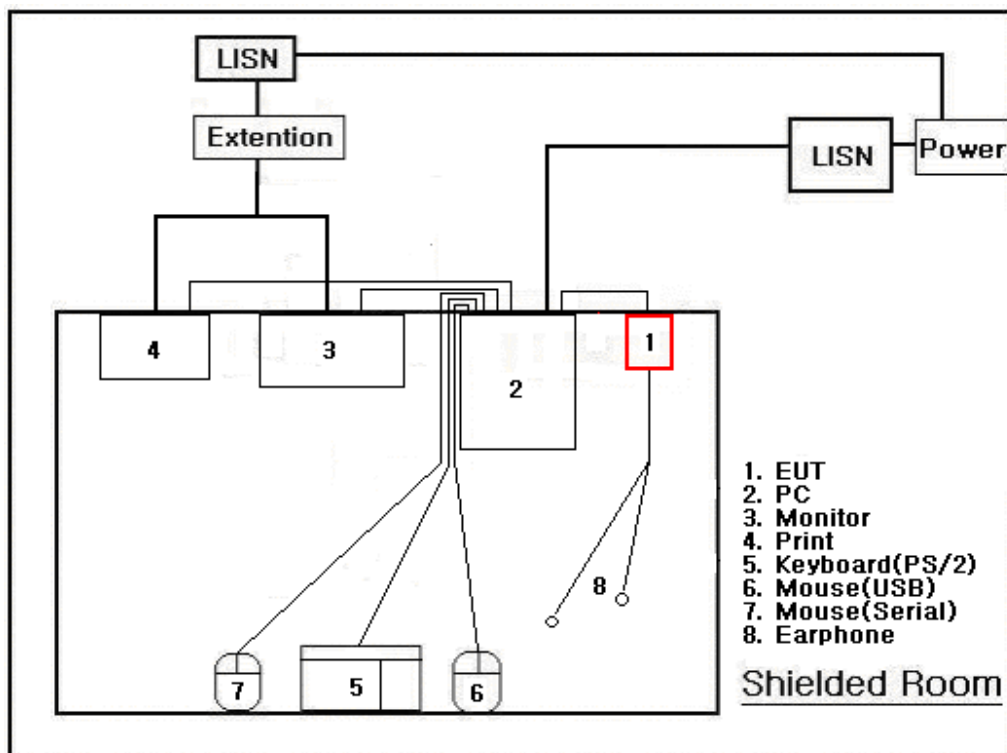
Conducted Emissions
