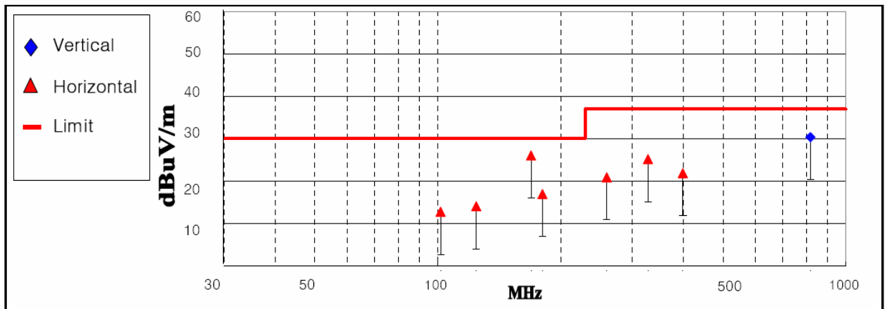
Fig 5. Graph of Radiated emission – Play Mode
