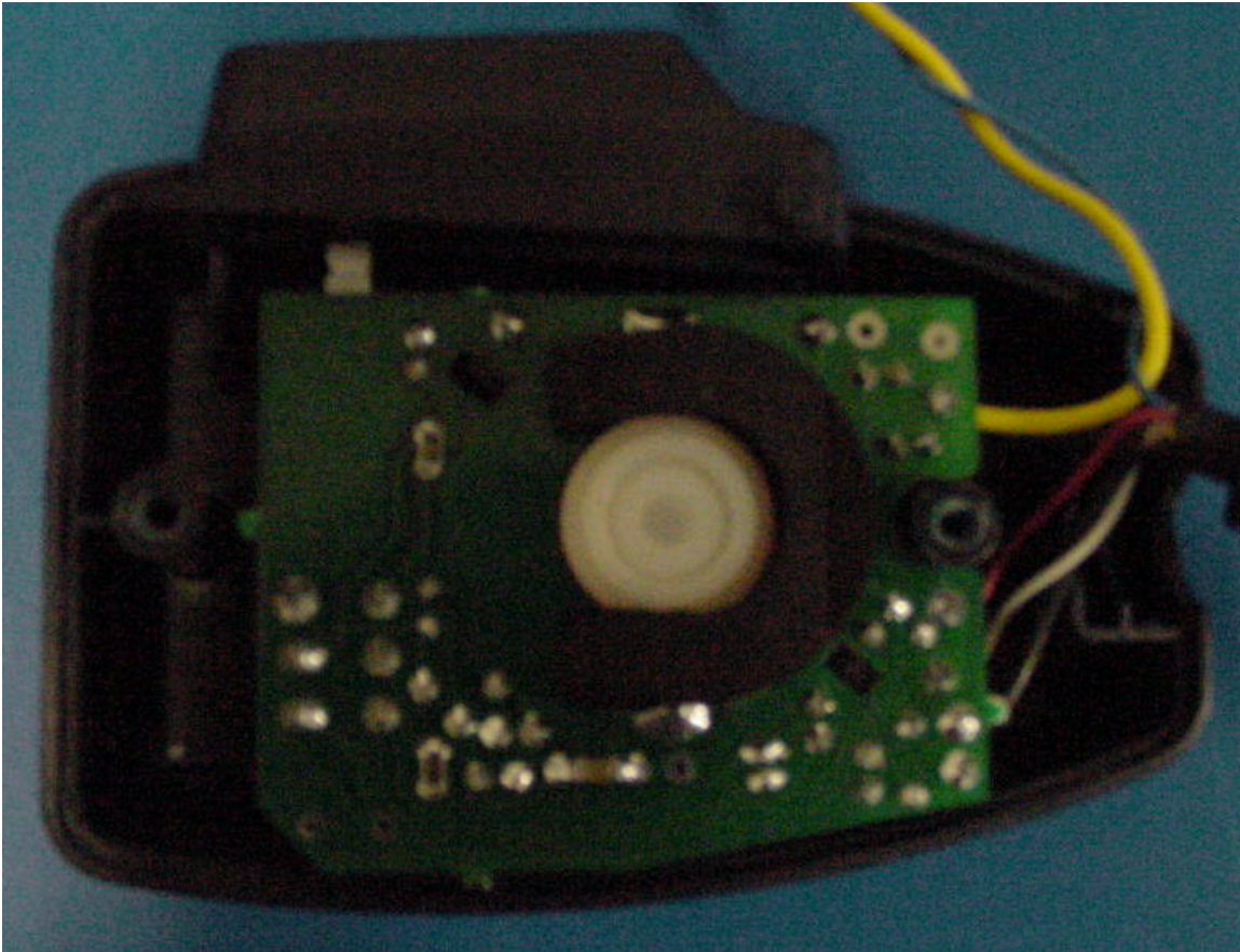
Handset showing PCB installed
