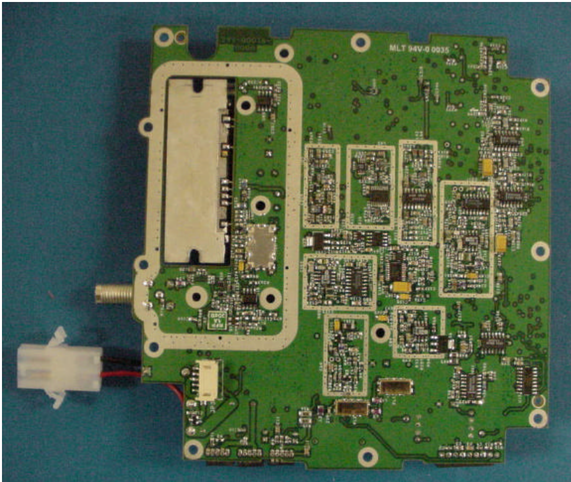
Bottom RF PCB
