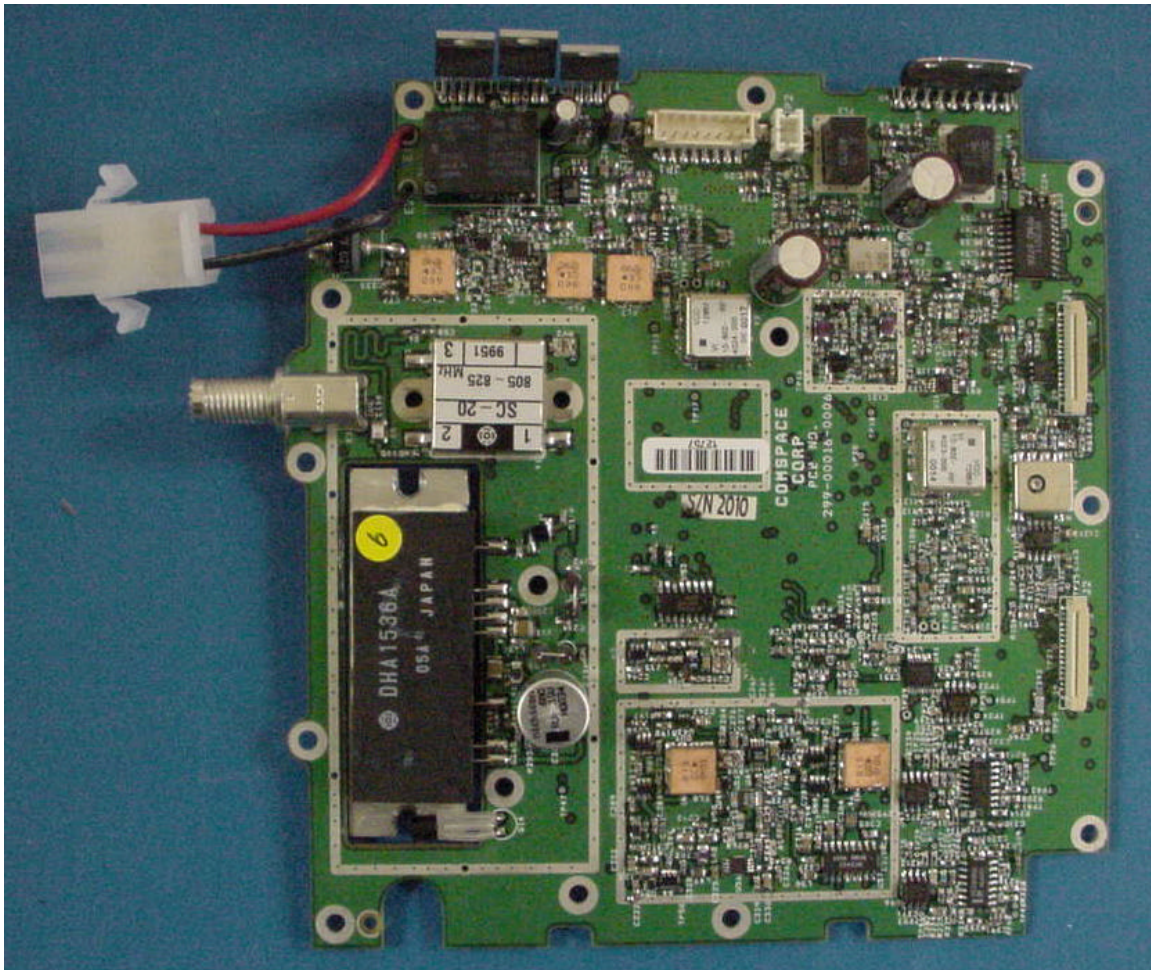
Top RF PCB
