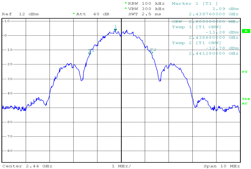
OBW Channel frequency: 2440 MHz
