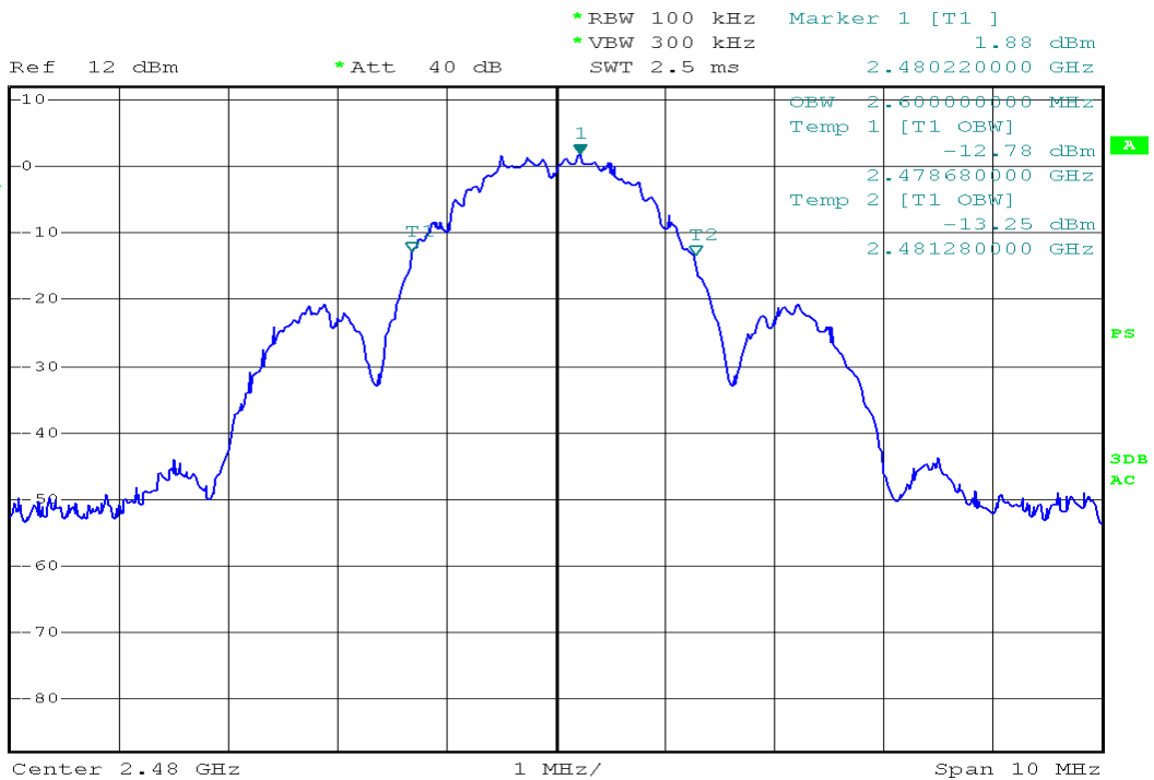
OBW Channel frequency: 2480 MHz
